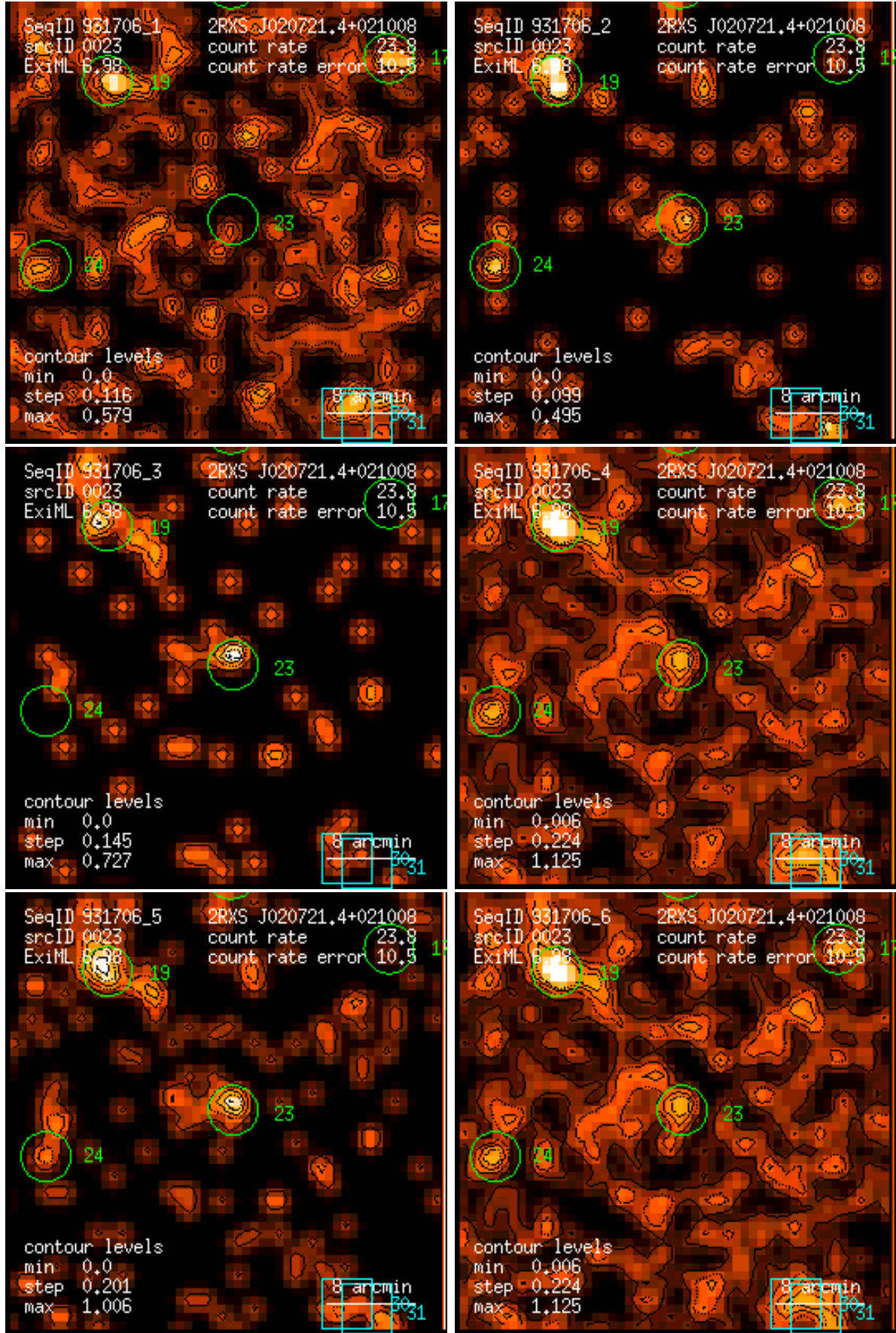
Figure 23: RASS 931706: detection 0023: band rate images, Gaussian filter: (1) PSPC channels 11 – 41, (2) 52 – 90, (3) 91 – 201, (4) 11 – 235, (5) 52 – 201, (6) 11 – 201. Broad band rates in counts/ks. Band rate contour levels in counts/ks/arcmin 2 .
