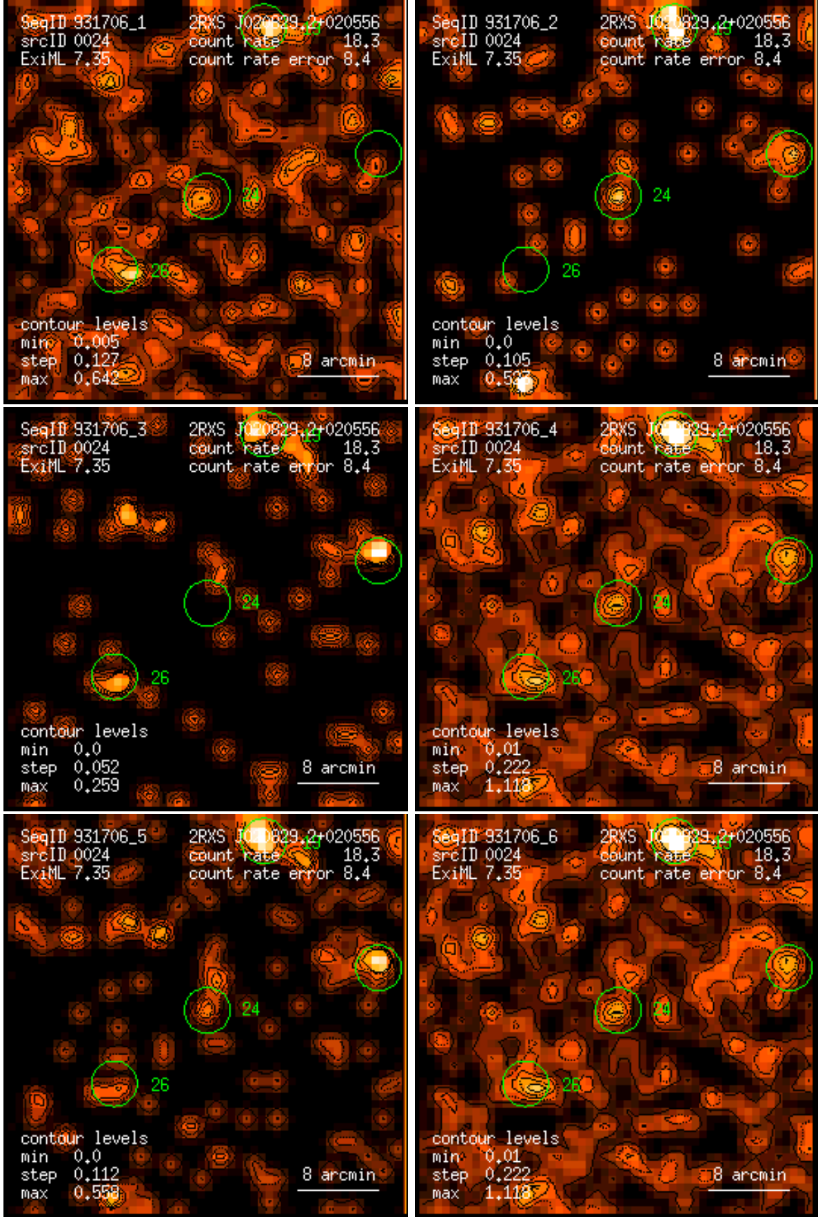
Figure 24: RASS 931706: detection 0024: band rate images, Gaussian filter: (1) PSPC channels 11 – 41, (2) 52 – 90, (3) 91 – 201, (4) 11 – 235, (5) 52 – 201, (6) 11 – 201. Broad band rates in counts/ks. Band rate contour levels in counts/ks/arcmin 2 .
