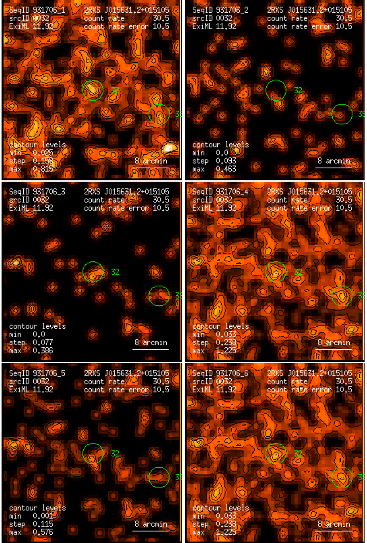
Figure 32: RASS 931706: detection 0032: band rate images, Gaussian filter: (1) PSPC channels 11 – 41, (2) 52 – 90, (3) 91 – 201, (4) 11 – 235, (5) 52 – 201, (6) 11 – 201. Broad band rates in counts/ks. Band rate contour levels in counts/ks/arcmin 2 .
