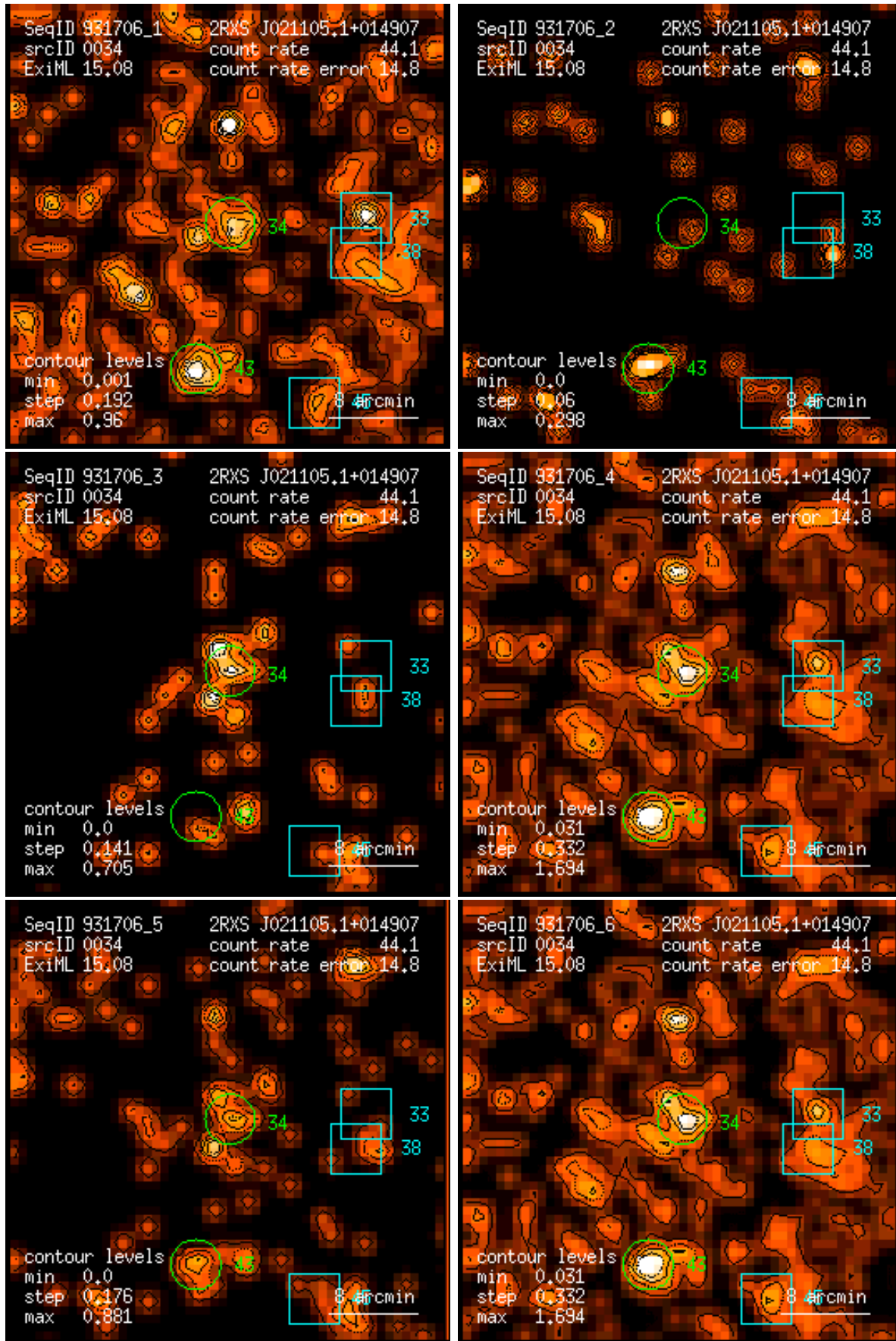
Figure 34: RASS 931706: detection 0034: band rate images, Gaussian filter: (1) PSPC channels 11 – 41, (2) 52 – 90, (3) 91 – 201, (4) 11 – 235, (5) 52 – 201, (6) 11 – 201. Broad band rates in counts/ks. Band rate contour levels in counts/ks/arcmin 2 .
