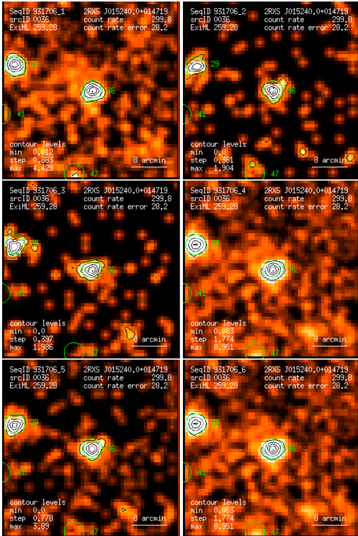
Figure 36: RASS 931706: detection 0036: band rate images, Gaussian filter: (1) PSPC channels 11 – 41, (2) 52 – 90, (3) 91 – 201, (4) 11 – 235, (5) 52 – 201, (6) 11 – 201. Broad band rates in counts/ks. Band rate contour levels in counts/ks/arcmin 2 .
