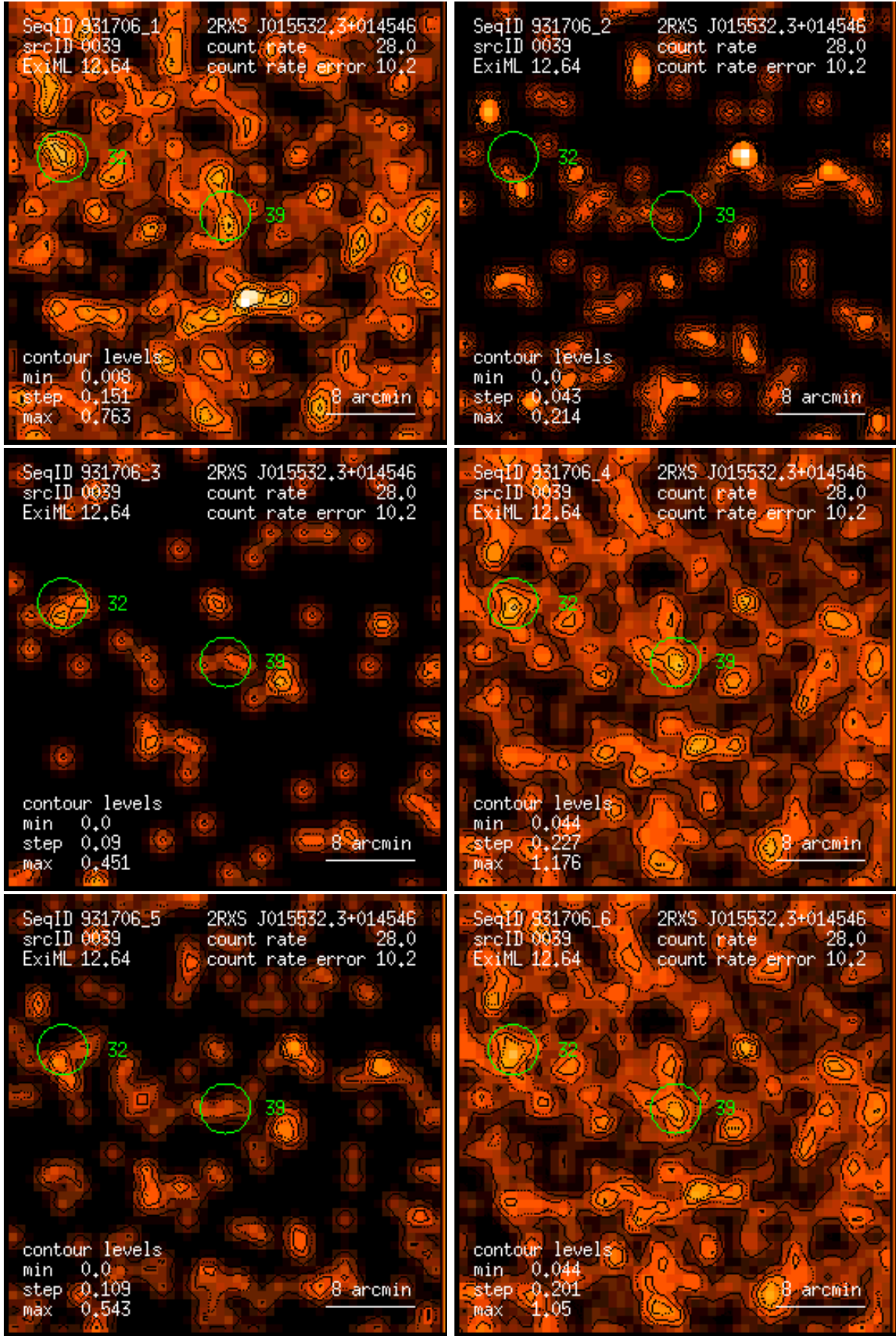
Figure 39: RASS 931706: detection 0039: band rate images, Gaussian filter: (1) PSPC channels 11 – 41, (2) 52 – 90, (3) 91 – 201, (4) 11 – 235, (5) 52 – 201, (6) 11 – 201. Broad band rates in counts/ks. Band rate contour levels in counts/ks/arcmin 2 .
