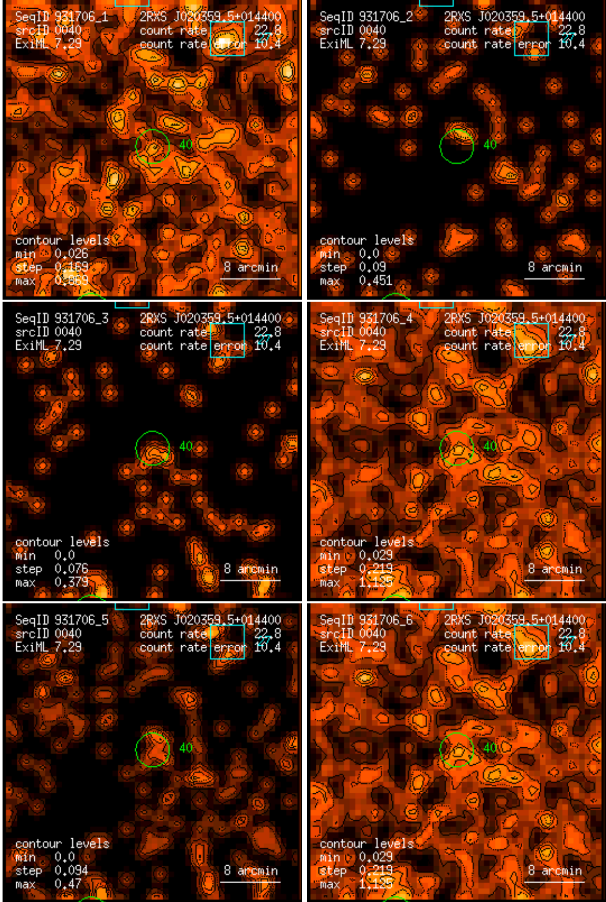
Figure 40: RASS 931706: detection 0040: band rate images, Gaussian filter: (1) PSPC channels 11 – 41, (2) 52 – 90, (3) 91 – 201, (4) 11 – 235, (5) 52 – 201, (6) 11 – 201. Broad band rates in counts/ks. Band rate contour levels in counts/ks/arcmin 2 .
