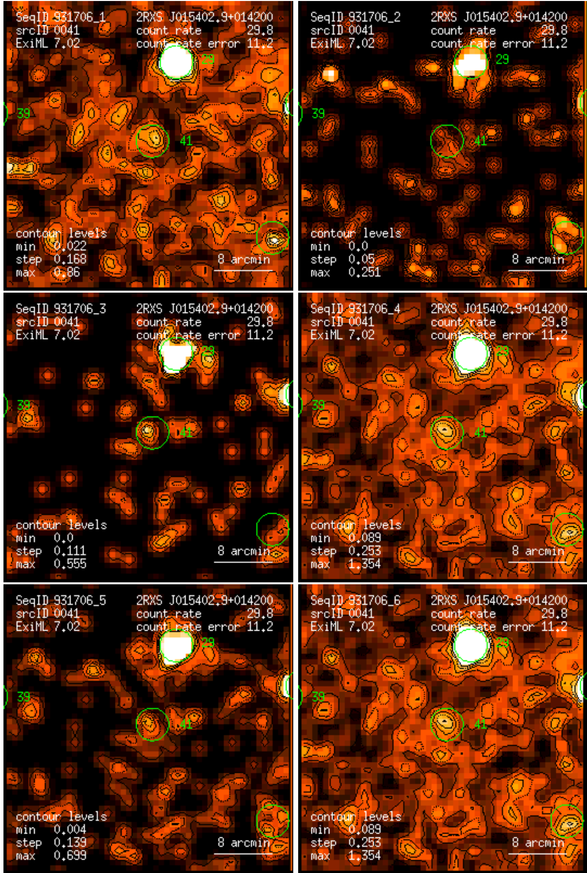
Figure 41: RASS 931706: detection 0041: band rate images, Gaussian filter: (1) PSPC channels 11 – 41, (2) 52 – 90, (3) 91 – 201, (4) 11 – 235, (5) 52 – 201, (6) 11 – 201. Broad band rates in counts/ks. Band rate contour levels in counts/ks/arcmin 2 .
