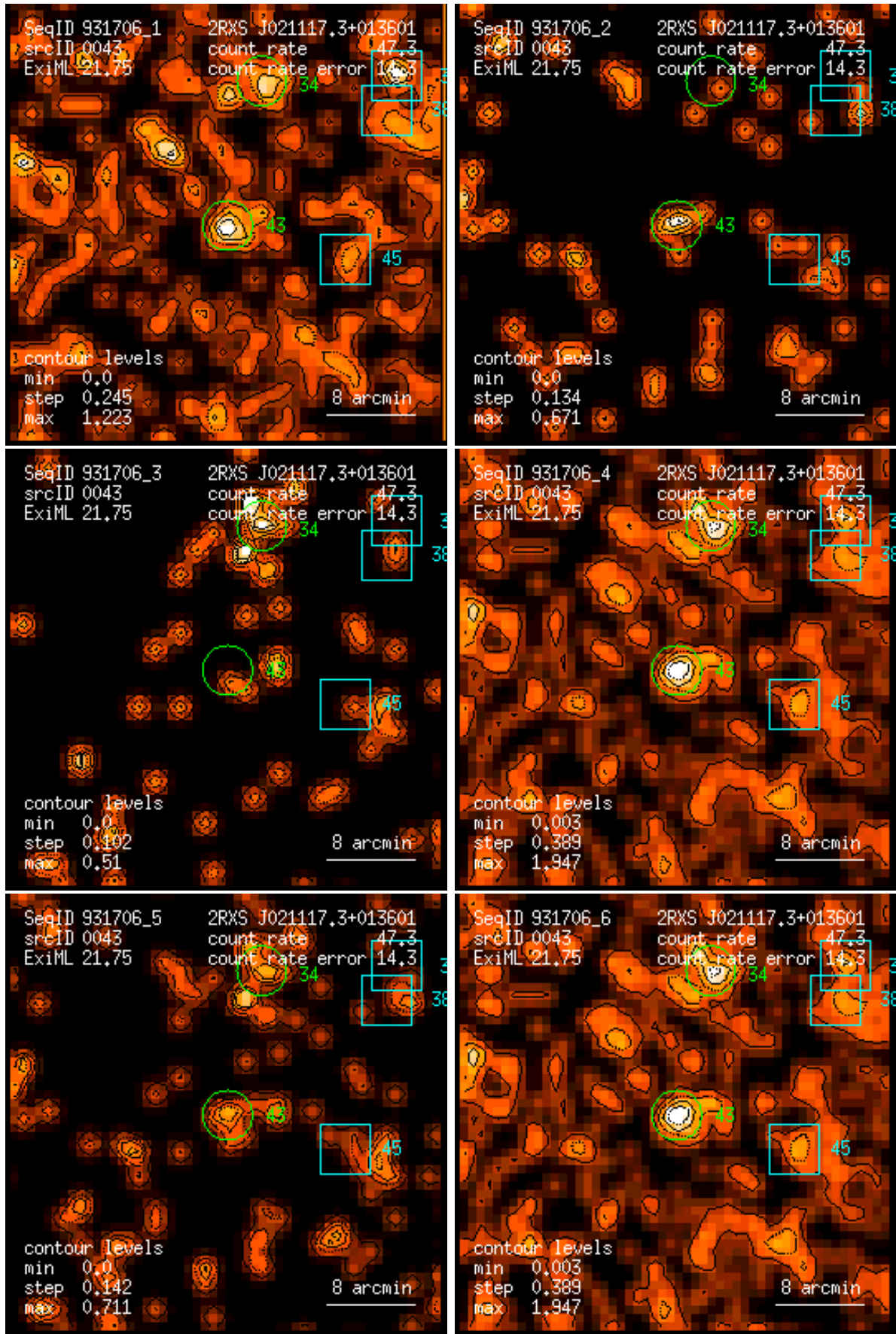
Figure 43: RASS 931706: detection 0043: band rate images, Gaussian filter: (1) PSPC channels 11 – 41, (2) 52 – 90, (3) 91 – 201, (4) 11 – 235, (5) 52 – 201, (6) 11 – 201. Broad band rates in counts/ks. Band rate contour levels in counts/ks/arcmin 2 .
