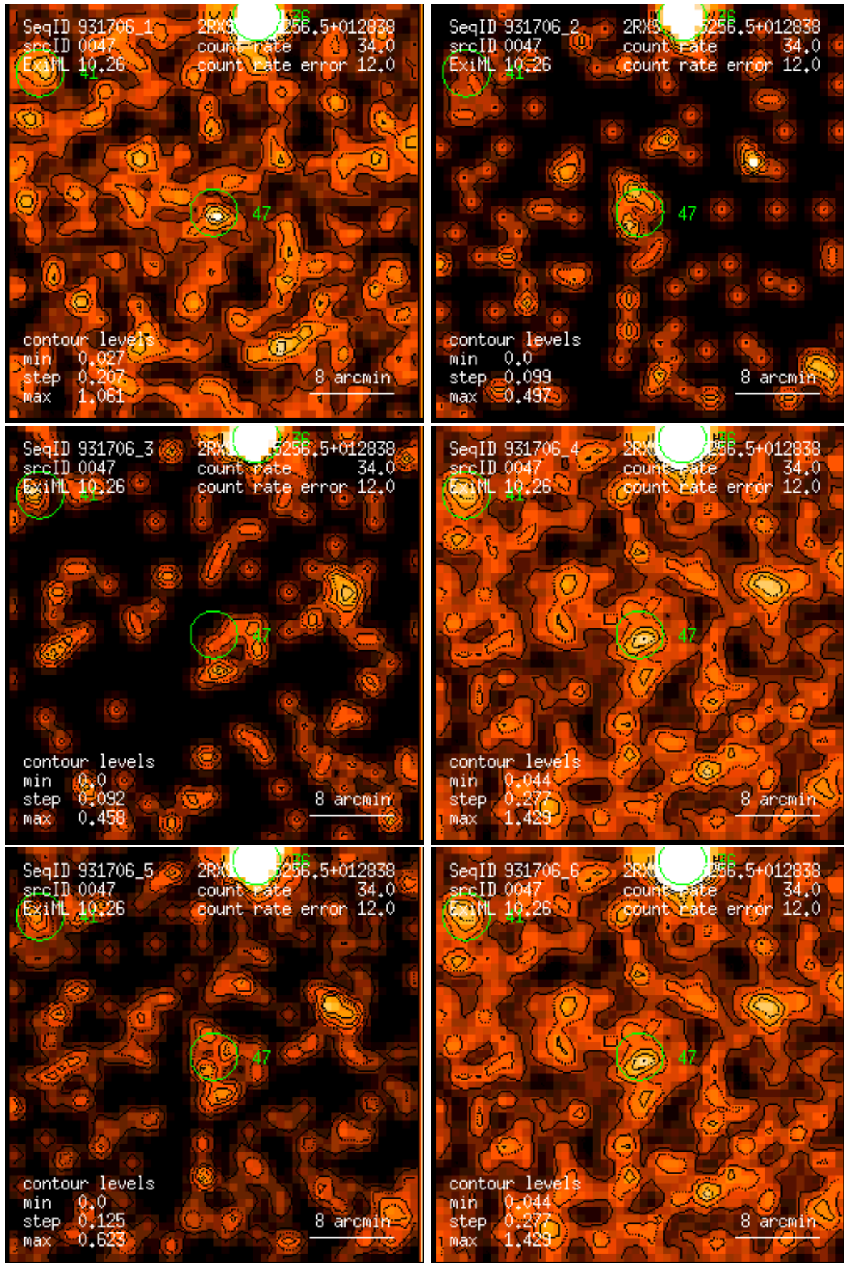
Figure 47: RASS 931706: detection 0047: band rate images, Gaussian filter: (1) PSPC channels 11 – 41, (2) 52 – 90, (3) 91 – 201, (4) 11 – 235, (5) 52 – 201, (6) 11 – 201. Broad band rates in counts/ks. Band rate contour levels in counts/ks/arcmin 2 .
