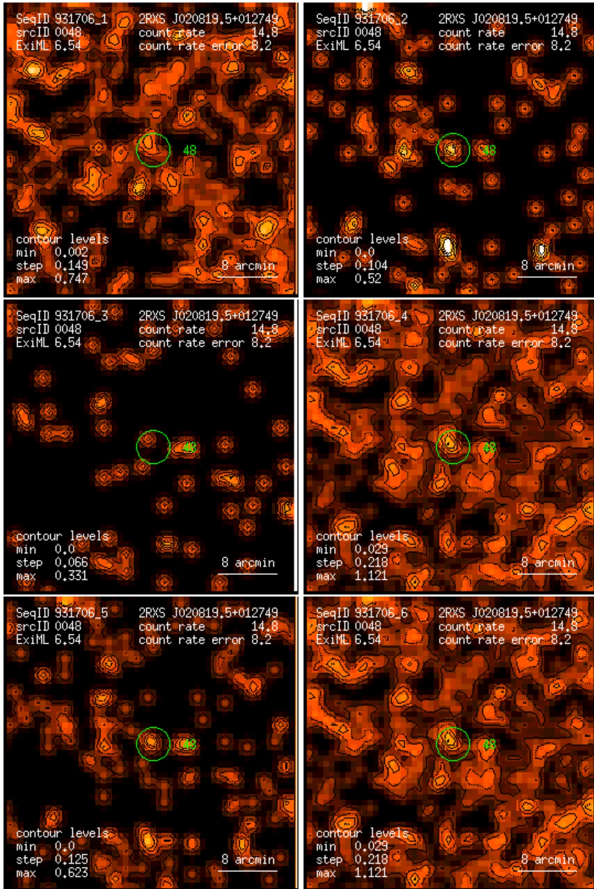
Figure 48: RASS 931706: detection 0048: band rate images, Gaussian filter: (1) PSPC channels 11 – 41, (2) 52 – 90, (3) 91 – 201, (4) 11 – 235, (5) 52 – 201, (6) 11 – 201. Broad band rates in counts/ks. Band rate contour levels in counts/ks/arcmin 2 .
