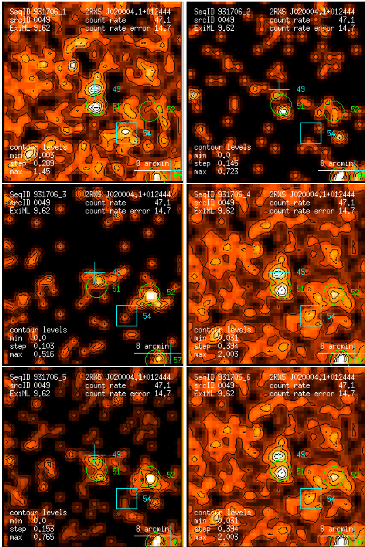
Figure 49: RASS 931706: detection 0049: band rate images, Gaussian filter: (1) PSPC channels 11 – 41, (2) 52 – 90, (3) 91 – 201, (4) 11 – 235, (5) 52 – 201, (6) 11 – 201. Broad band rates in counts/ks. Band rate contour levels in counts/ks/arcmin 2 .
