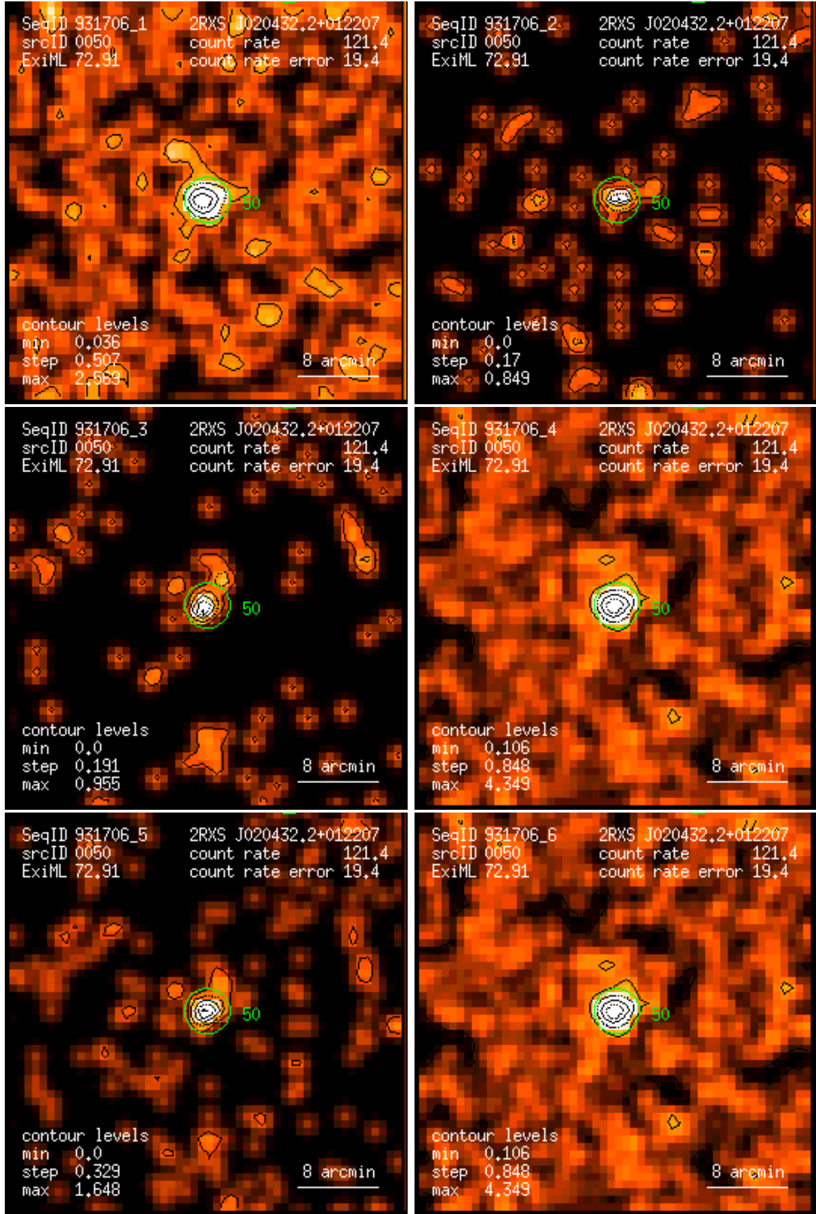
Figure 50: RASS 931706: detection 0050: band rate images, Gaussian filter: (1) PSPC channels 11 – 41, (2) 52 – 90, (3) 91 – 201, (4) 11 – 235, (5) 52 – 201, (6) 11 – 201. Broad band rates in counts/ks. Band rate contour levels in counts/ks/arcmin 2 .
