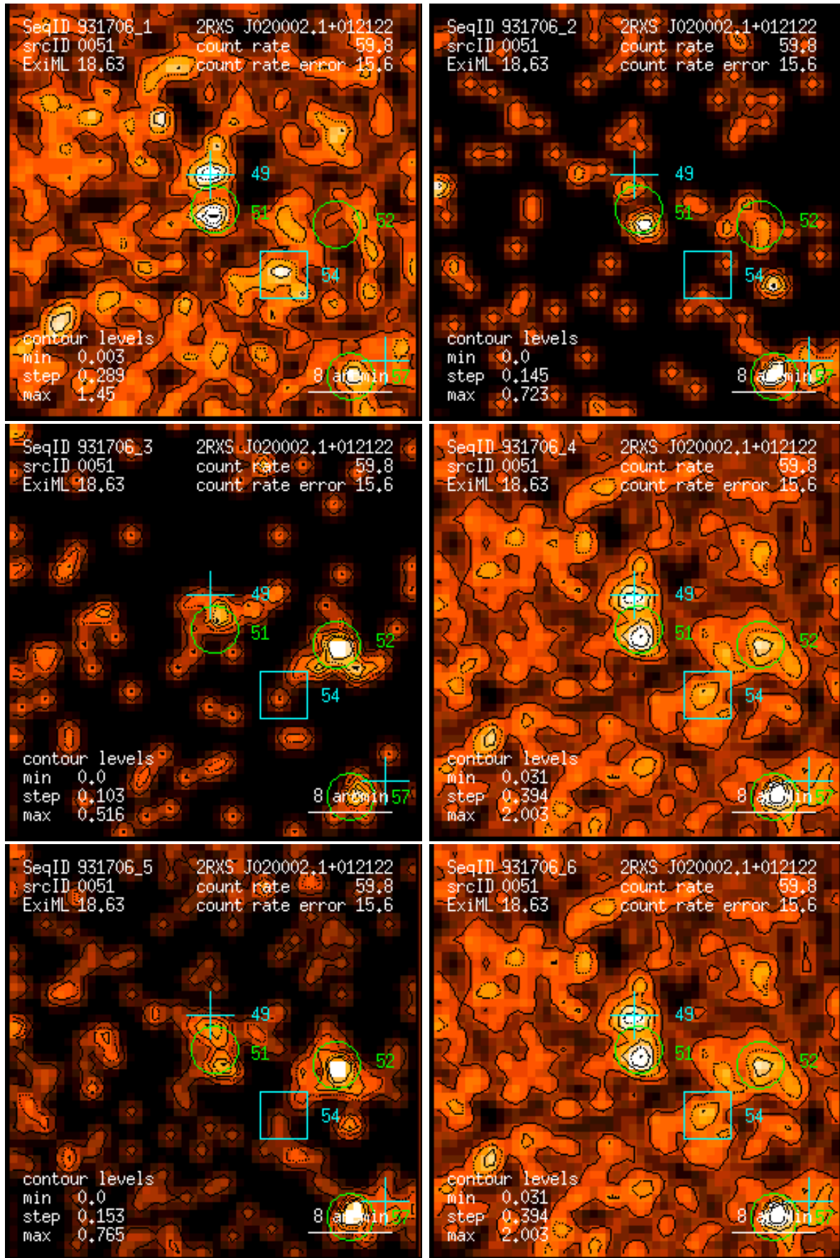
Figure 51: RASS 931706: detection 0051: band rate images, Gaussian filter: (1) PSPC channels 11 – 41, (2) 52 – 90, (3) 91 – 201, (4) 11 – 235, (5) 52 – 201, (6) 11 – 201. Broad band rates in counts/ks. Band rate contour levels in counts/ks/arcmin 2 .
