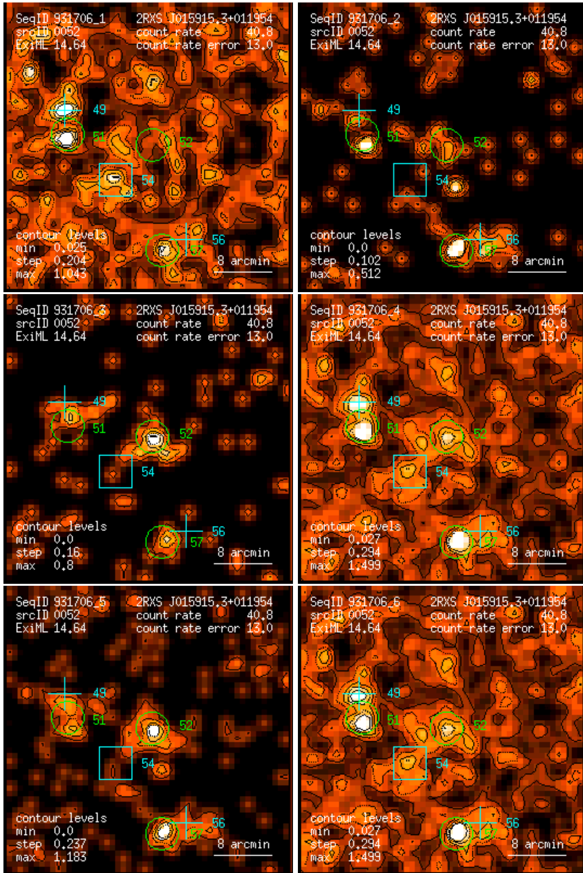
Figure 52: RASS 931706: detection 0052: band rate images, Gaussian filter: (1) PSPC channels 11 – 41, (2) 52 – 90, (3) 91 – 201, (4) 11 – 235, (5) 52 – 201, (6) 11 – 201. Broad band rates in counts/ks. Band rate contour levels in counts/ks/arcmin 2 .
