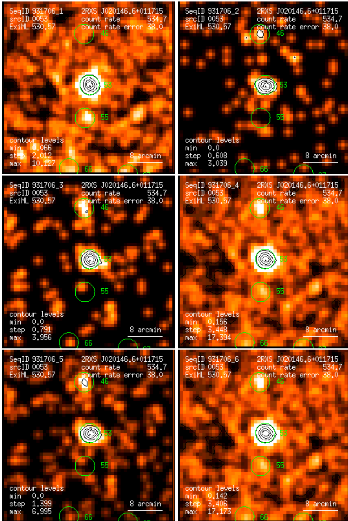
Figure 53: RASS 931706: detection 0053: band rate images, Gaussian filter: (1) PSPC channels 11 – 41, (2) 52 – 90, (3) 91 – 201, (4) 11 – 235, (5) 52 – 201, (6) 11 – 201. Broad band rates in counts/ks. Band rate contour levels in counts/ks/arcmin 2 .
