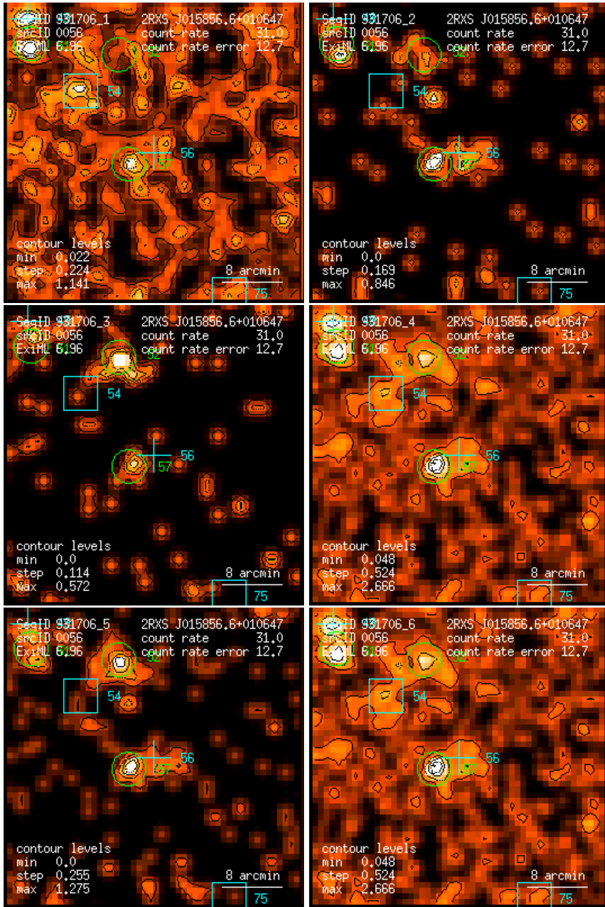
Figure 56: RASS 931706: detection 0056: band rate images, Gaussian filter: (1) PSPC channels 11 – 41, (2) 52 – 90, (3) 91 – 201, (4) 11 – 235, (5) 52 – 201, (6) 11 – 201. Broad band rates in counts/ks. Band rate contour levels in counts/ks/arcmin 2 .
