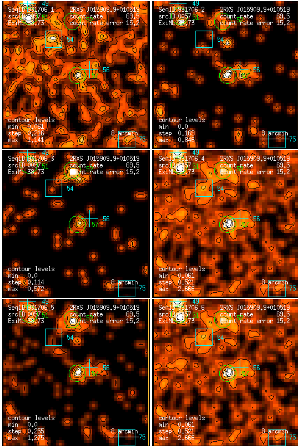
Figure 57: RASS 931706: detection 0057: band rate images, Gaussian filter: (1) PSPC channels 11 – 41, (2) 52 – 90, (3) 91 – 201, (4) 11 – 235, (5) 52 – 201, (6) 11 – 201. Broad band rates in counts/ks. Band rate contour levels in counts/ks/arcmin 2 .
