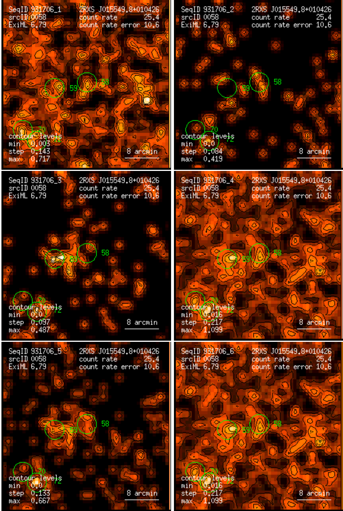
Figure 58: RASS 931706: detection 0058: band rate images, Gaussian filter: (1) PSPC channels 11 – 41, (2) 52 – 90, (3) 91 – 201, (4) 11 – 235, (5) 52 – 201, (6) 11 – 201. Broad band rates in counts/ks. Band rate contour levels in counts/ks/arcmin 2 .
