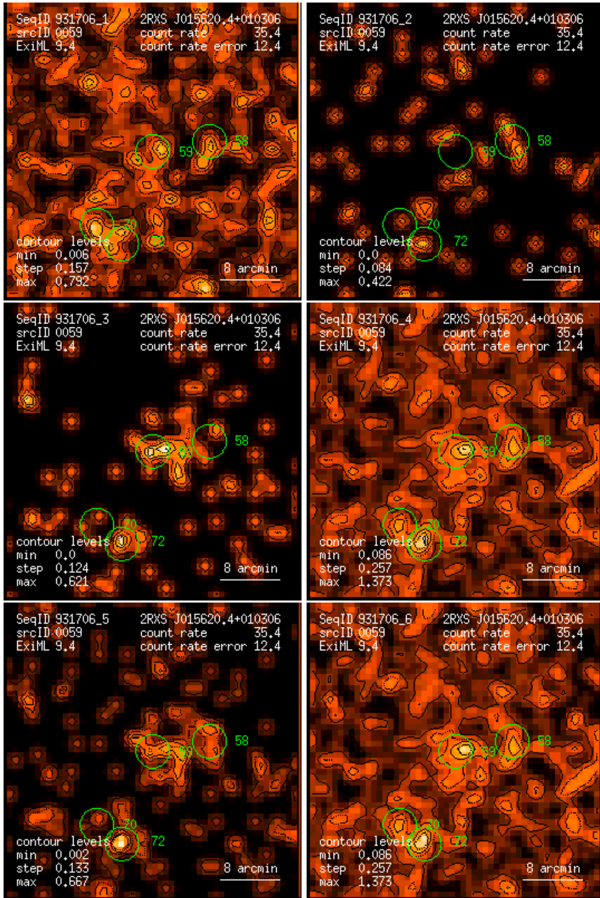
Figure 59: RASS 931706: detection 0059: band rate images, Gaussian filter: (1) PSPC channels 11 – 41, (2) 52 – 90, (3) 91 – 201, (4) 11 – 235, (5) 52 – 201, (6) 11 – 201. Broad band rates in counts/ks. Band rate contour levels in counts/ks/arcmin 2 .
