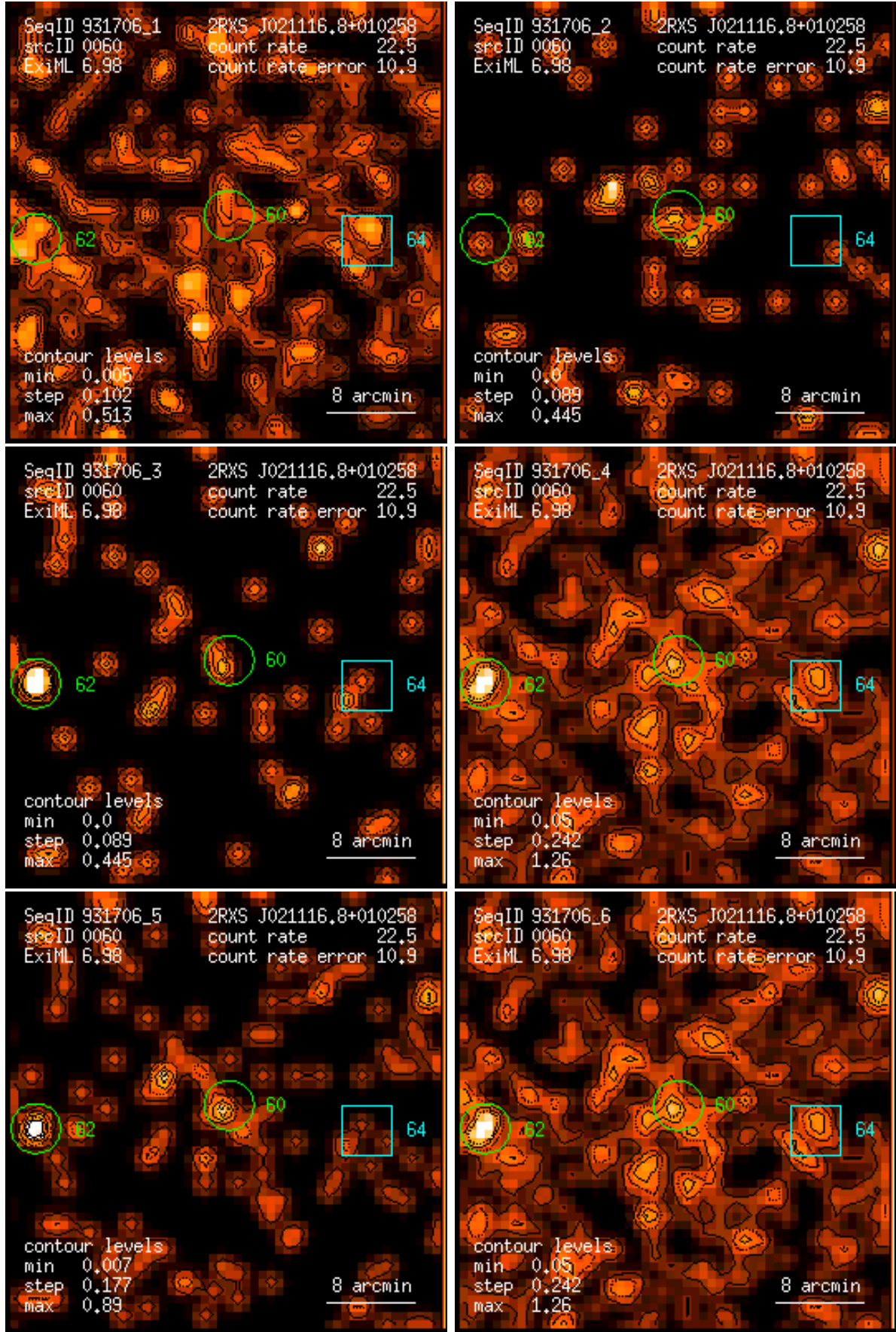
Figure 60: RASS 931706: detection 0060: band rate images, Gaussian filter: (1) PSPC channels 11 – 41, (2) 52 – 90, (3) 91 – 201, (4) 11 – 235, (5) 52 – 201, (6) 11 – 201. Broad band rates in counts/ks. Band rate contour levels in counts/ks/arcmin 2 .
