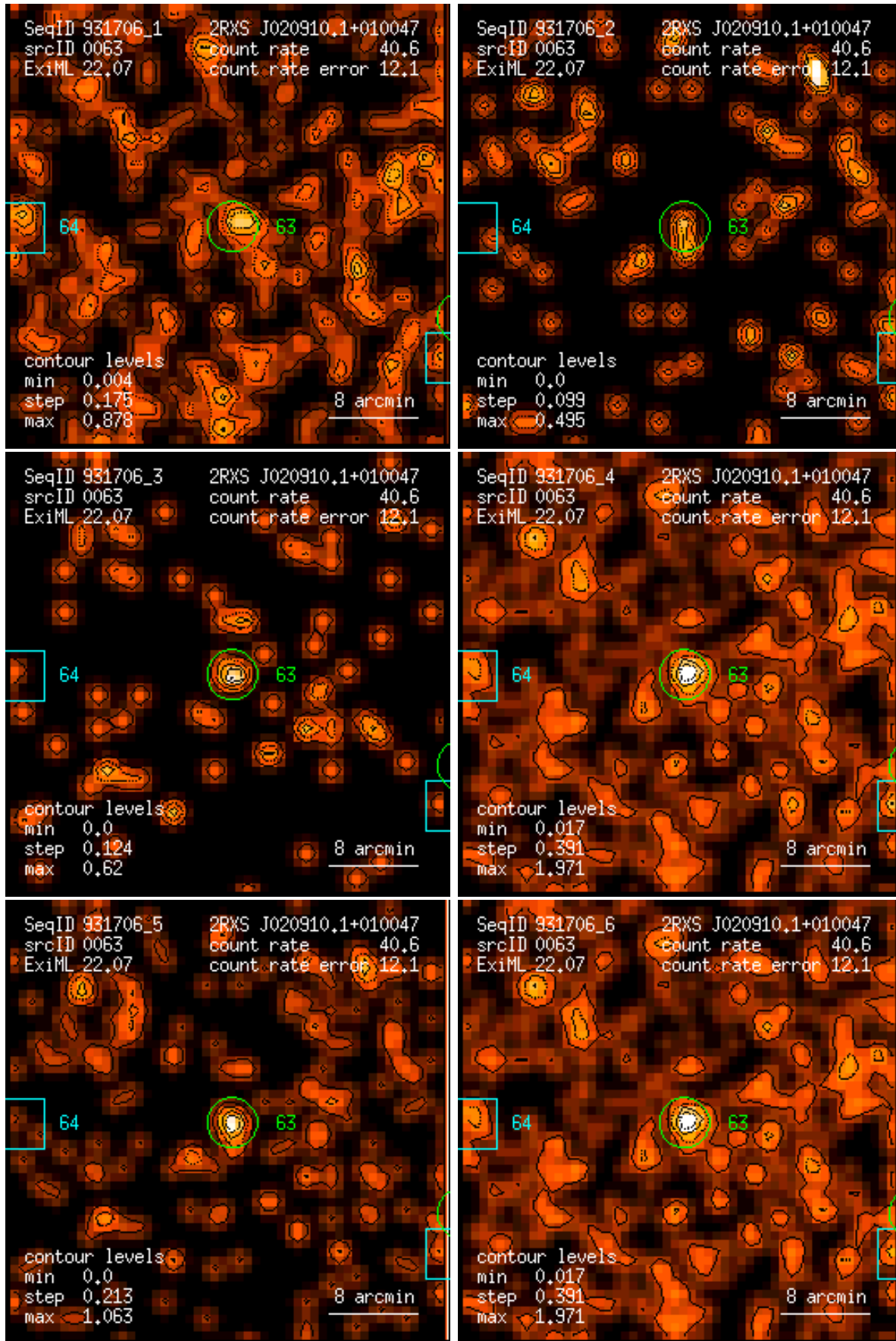
Figure 63: RASS 931706: detection 0063: band rate images, Gaussian filter: (1) PSPC channels 11 – 41, (2) 52 – 90, (3) 91 – 201, (4) 11 – 235, (5) 52 – 201, (6) 11 – 201. Broad band rates in counts/ks. Band rate contour levels in counts/ks/arcmin 2 .
