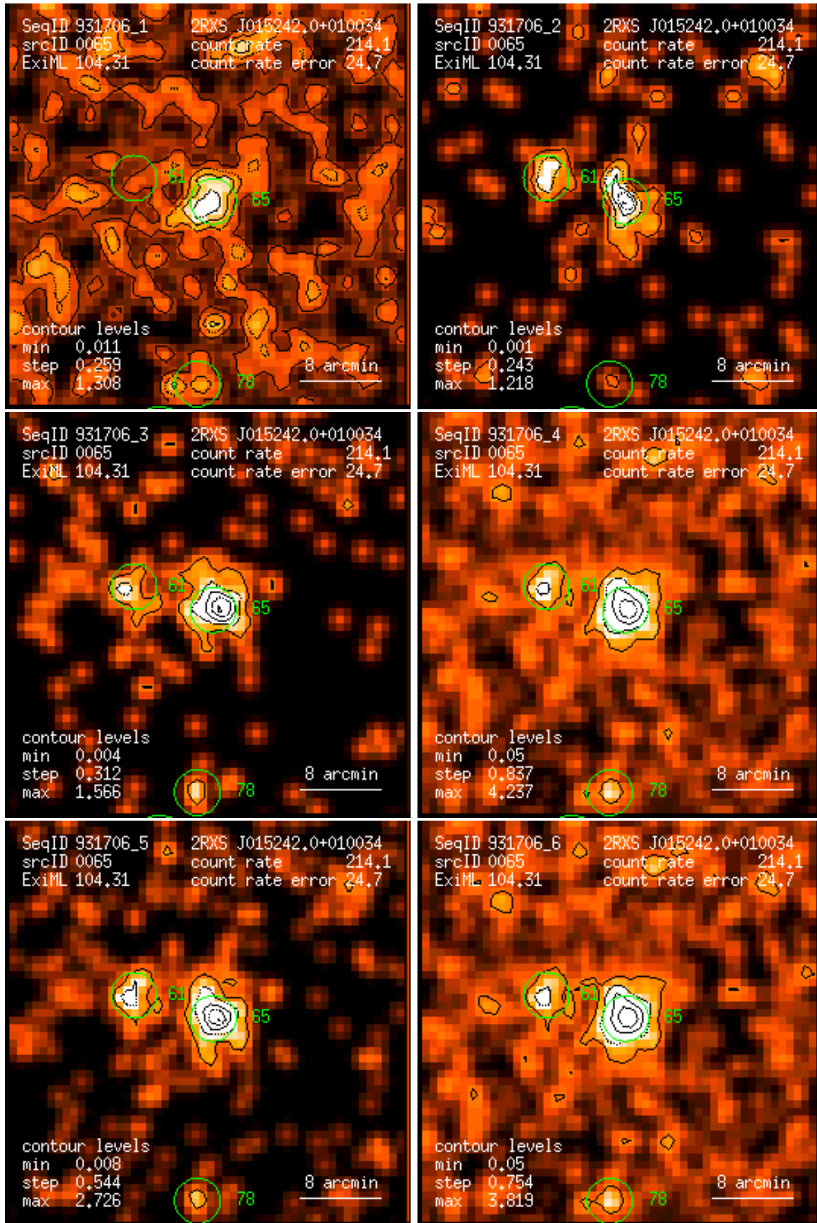
Figure 65: RASS 931706: detection 0065: band rate images, Gaussian filter: (1) PSPC channels 11 – 41, (2) 52 – 90, (3) 91 – 201, (4) 11 – 235, (5) 52 – 201, (6) 11 – 201. Broad band rates in counts/ks. Band rate contour levels in counts/ks/arcmin 2 .
