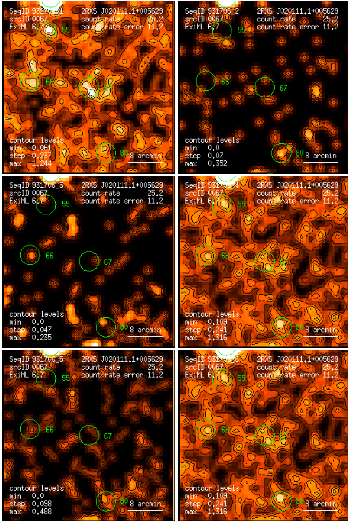
Figure 67: RASS 931706: detection 0067: band rate images, Gaussian filter: (1) PSPC channels 11 – 41, (2) 52 – 90, (3) 91 – 201, (4) 11 – 235, (5) 52 – 201, (6) 11 – 201. Broad band rates in counts/ks. Band rate contour levels in counts/ks/arcmin 2 .
