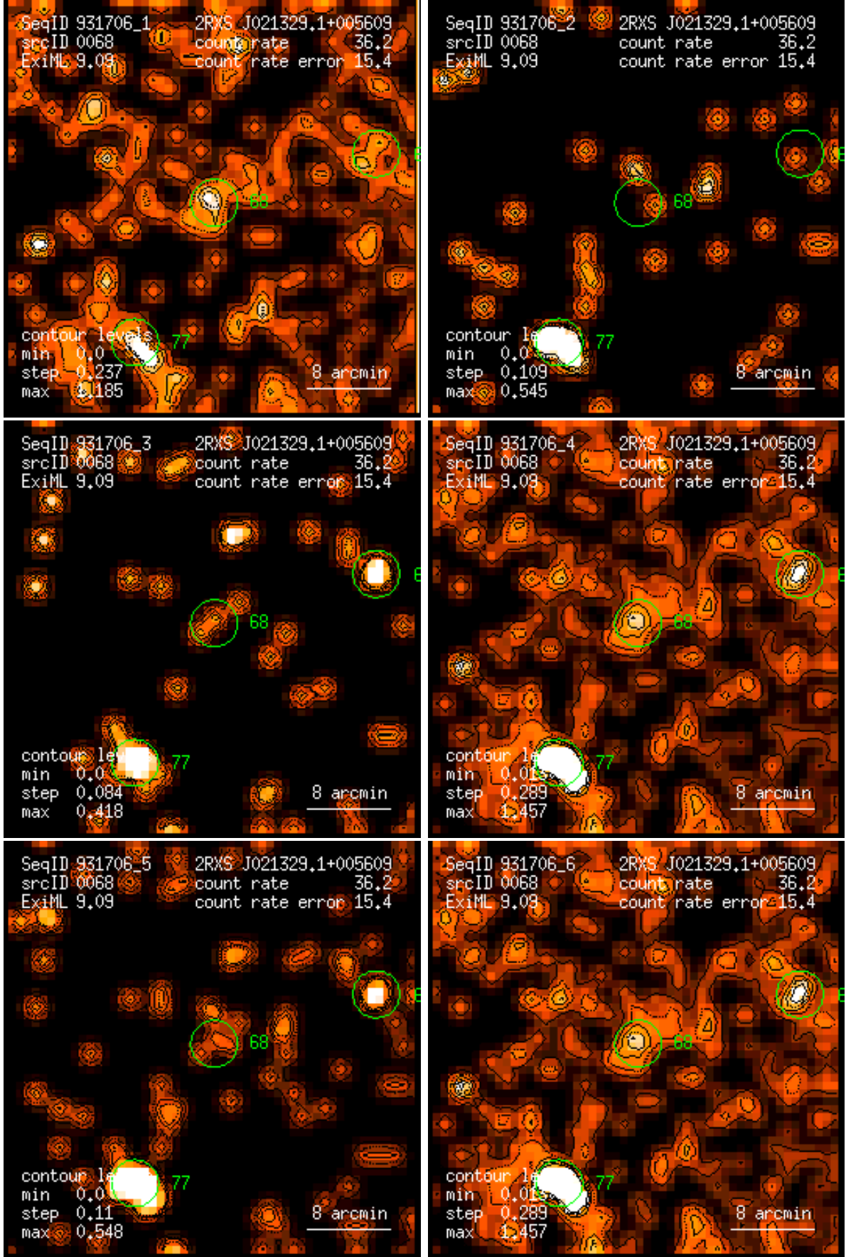
Figure 68: RASS 931706: detection 0068: band rate images, Gaussian filter: (1) PSPC channels 11 – 41, (2) 52 – 90, (3) 91 – 201, (4) 11 – 235, (5) 52 – 201, (6) 11 – 201. Broad band rates in counts/ks. Band rate contour levels in counts/ks/arcmin 2 .
