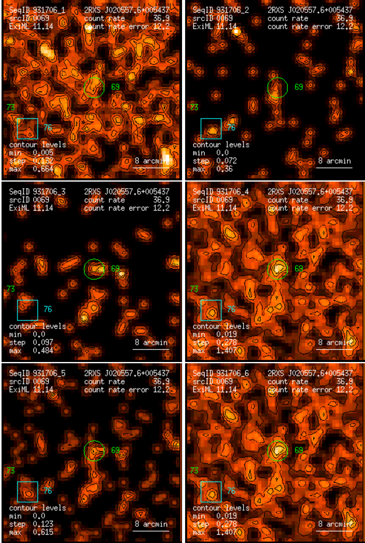
Figure 69: RASS 931706: detection 0069: band rate images, Gaussian filter: (1) PSPC channels 11 – 41, (2) 52 – 90, (3) 91 – 201, (4) 11 – 235, (5) 52 – 201, (6) 11 – 201. Broad band rates in counts/ks. Band rate contour levels in counts/ks/arcmin 2 .
