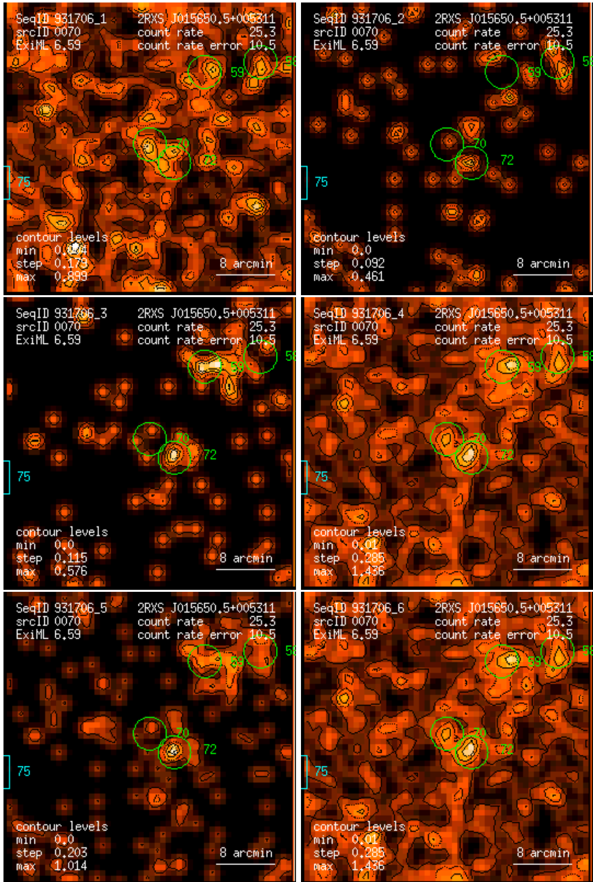
Figure 70: RASS 931706: detection 0070: band rate images, Gaussian filter: (1) PSPC channels 11 – 41, (2) 52 – 90, (3) 91 – 201, (4) 11 – 235, (5) 52 – 201, (6) 11 – 201. Broad band rates in counts/ks. Band rate contour levels in counts/ks/arcmin 2 .
