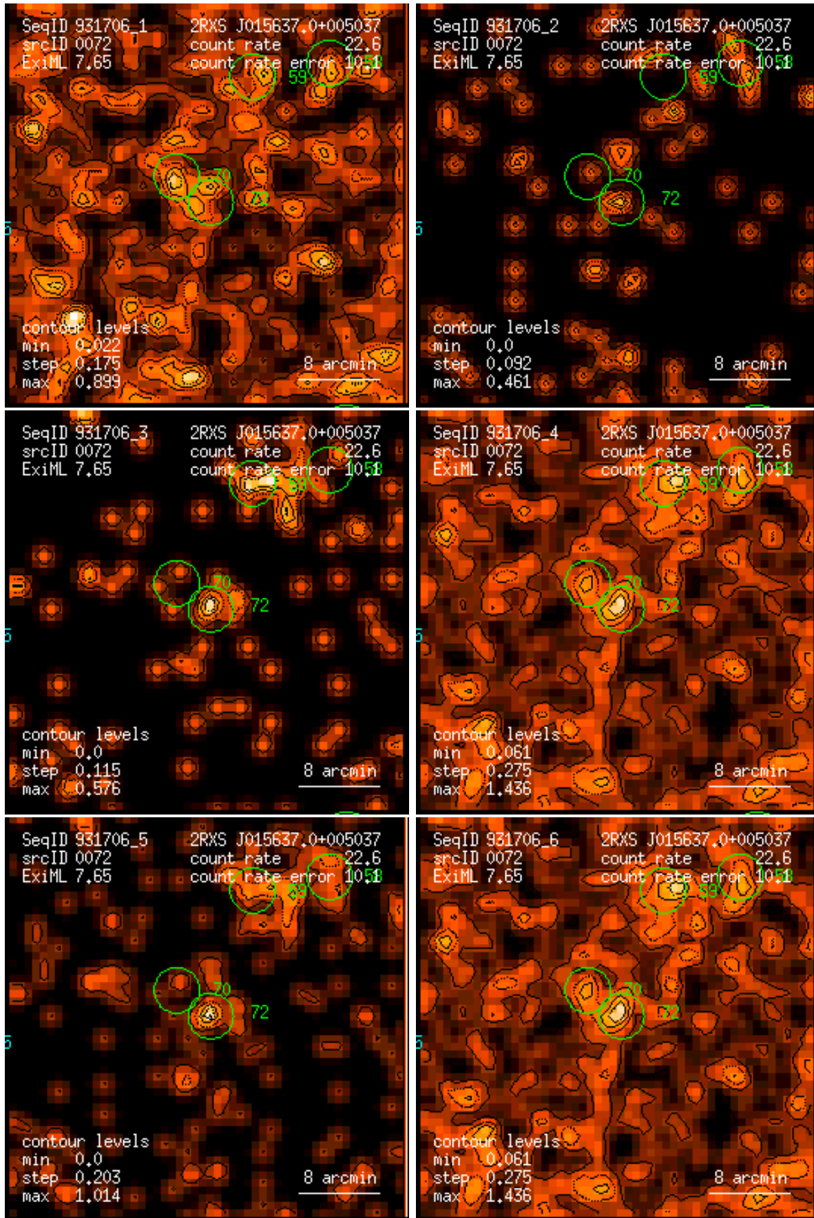
Figure 72: RASS 931706: detection 0072: band rate images, Gaussian filter: (1) PSPC channels 11 – 41, (2) 52 – 90, (3) 91 – 201, (4) 11 – 235, (5) 52 – 201, (6) 11 – 201. Broad band rates in counts/ks. Band rate contour levels in counts/ks/arcmin 2 .
