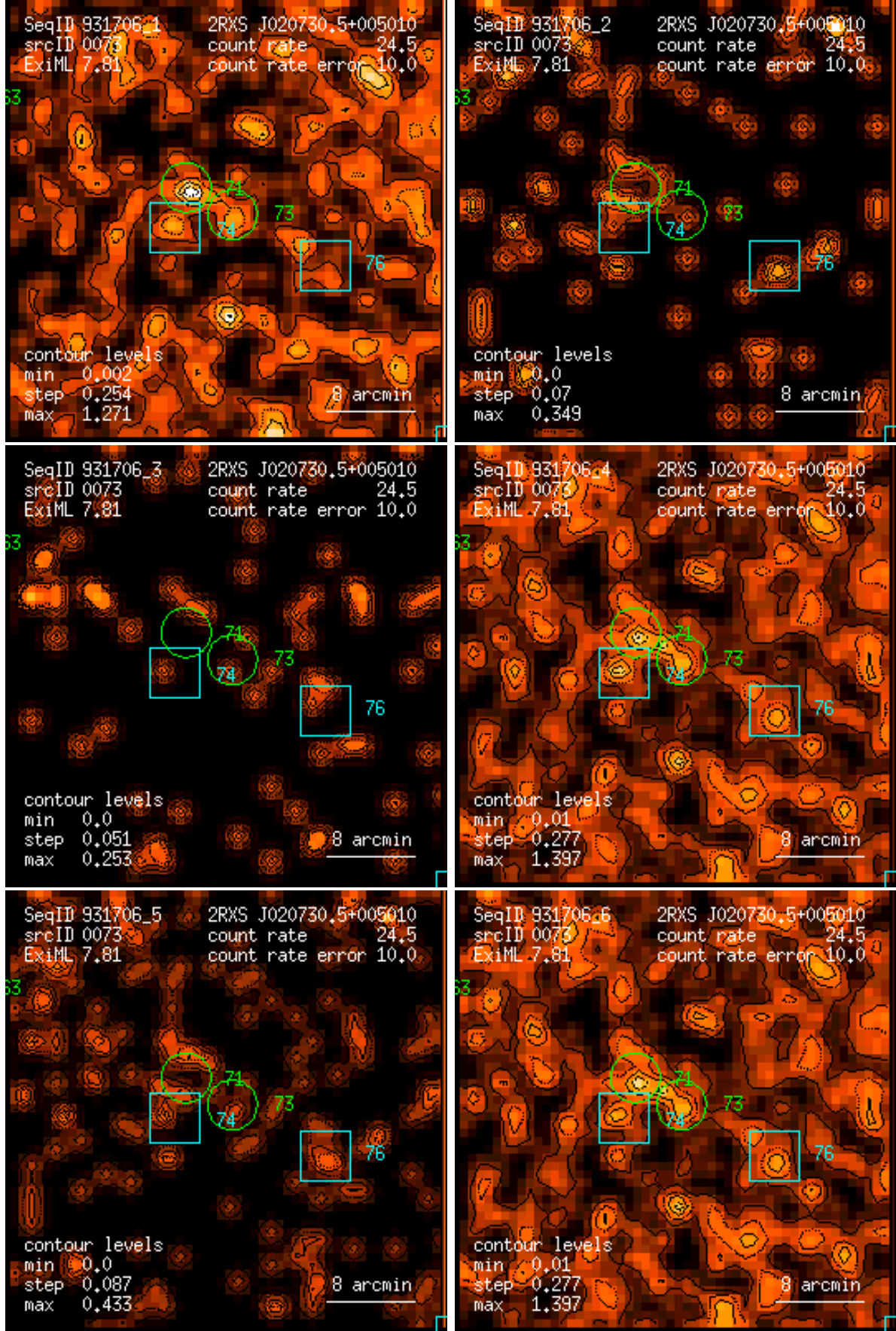
Figure 73: RASS 931706: detection 0073: band rate images, Gaussian filter: (1) PSPC channels 11 – 41, (2) 52 – 90, (3) 91 – 201, (4) 11 – 235, (5) 52 – 201, (6) 11 – 201. Broad band rates in counts/ks. Band rate contour levels in counts/ks/arcmin 2 .
