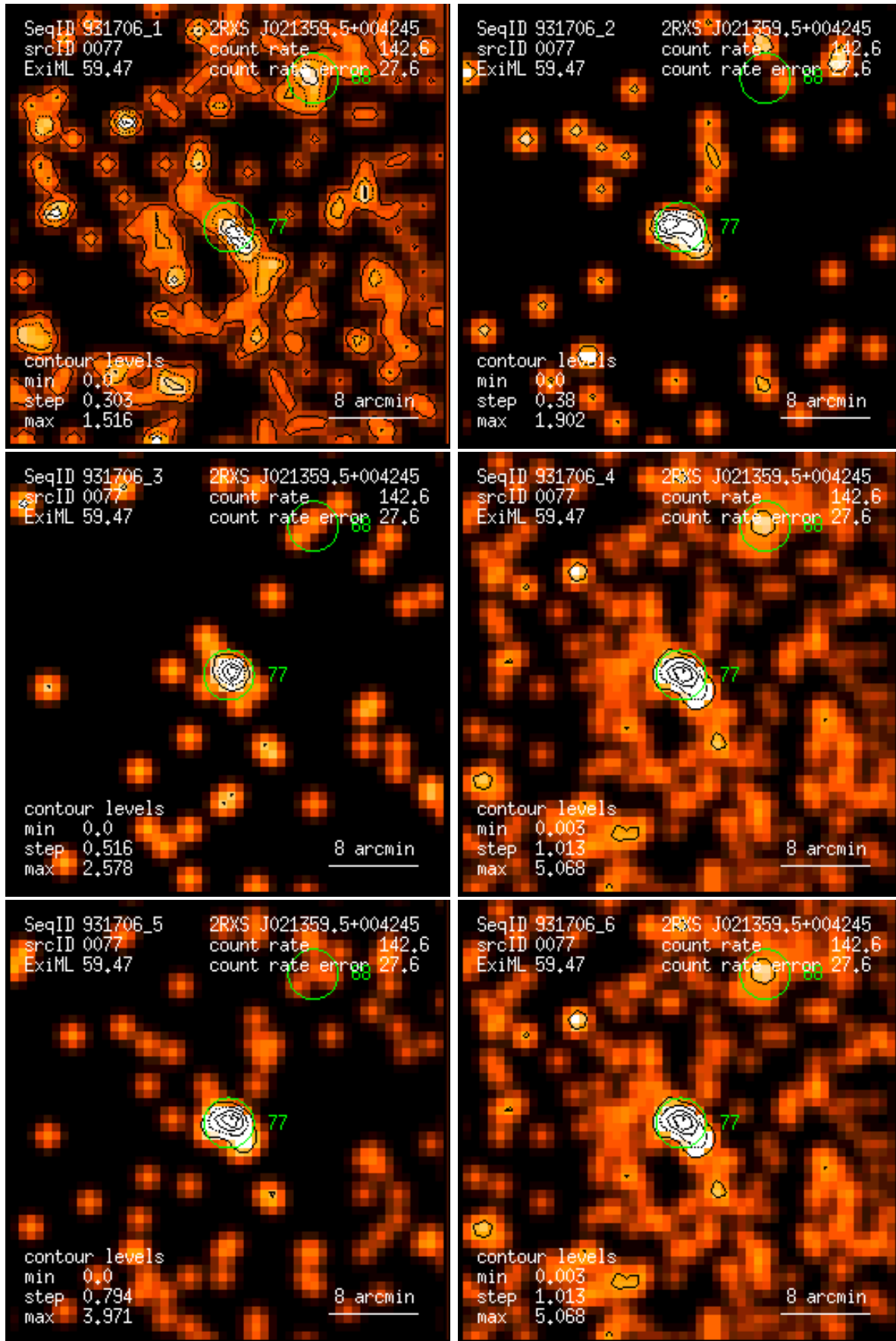
Figure 77: RASS 931706: detection 0077: band rate images, Gaussian filter: (1) PSPC channels 11 – 41, (2) 52 – 90, (3) 91 – 201, (4) 11 – 235, (5) 52 – 201, (6) 11 – 201. Broad band rates in counts/ks. Band rate contour levels in counts/ks/arcmin 2 .
