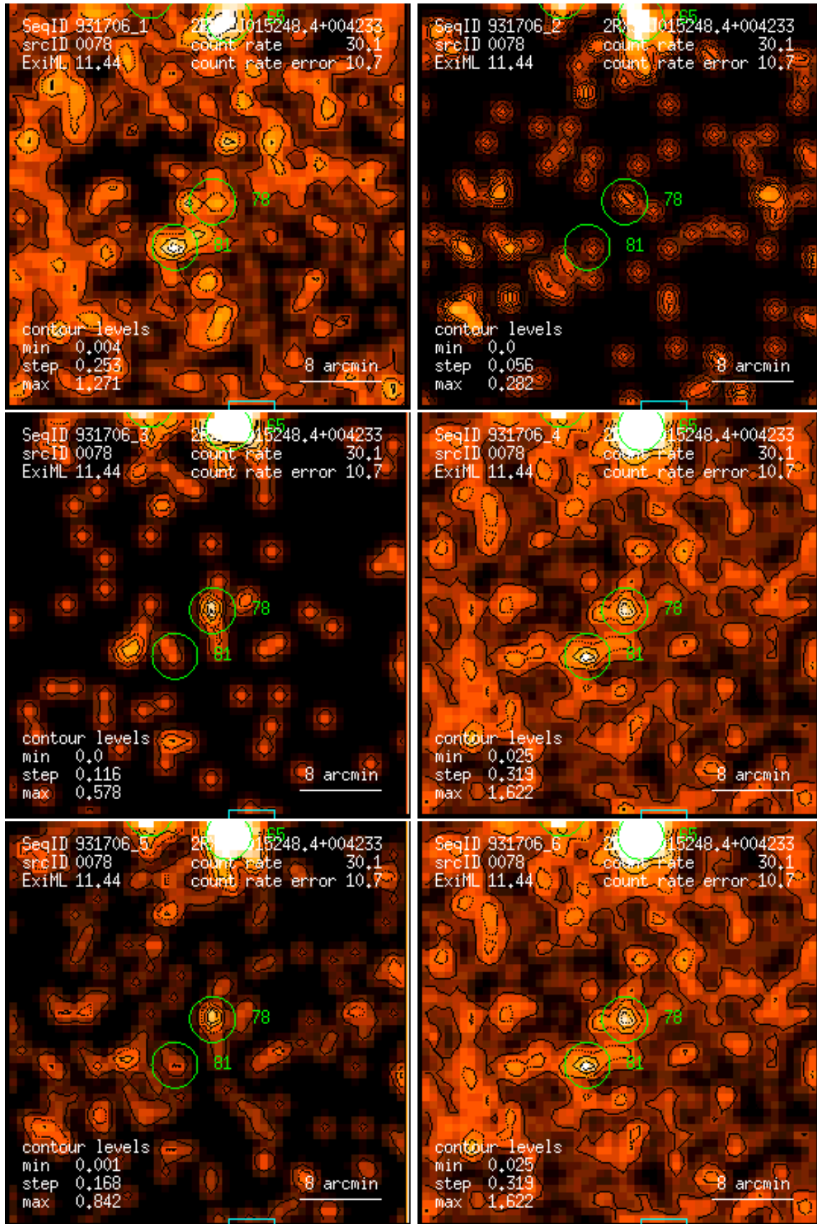
Figure 78: RASS 931706: detection 0078: band rate images, Gaussian filter: (1) PSPC channels 11 – 41, (2) 52 – 90, (3) 91 – 201, (4) 11 – 235, (5) 52 – 201, (6) 11 – 201. Broad band rates in counts/ks. Band rate contour levels in counts/ks/arcmin 2 .
