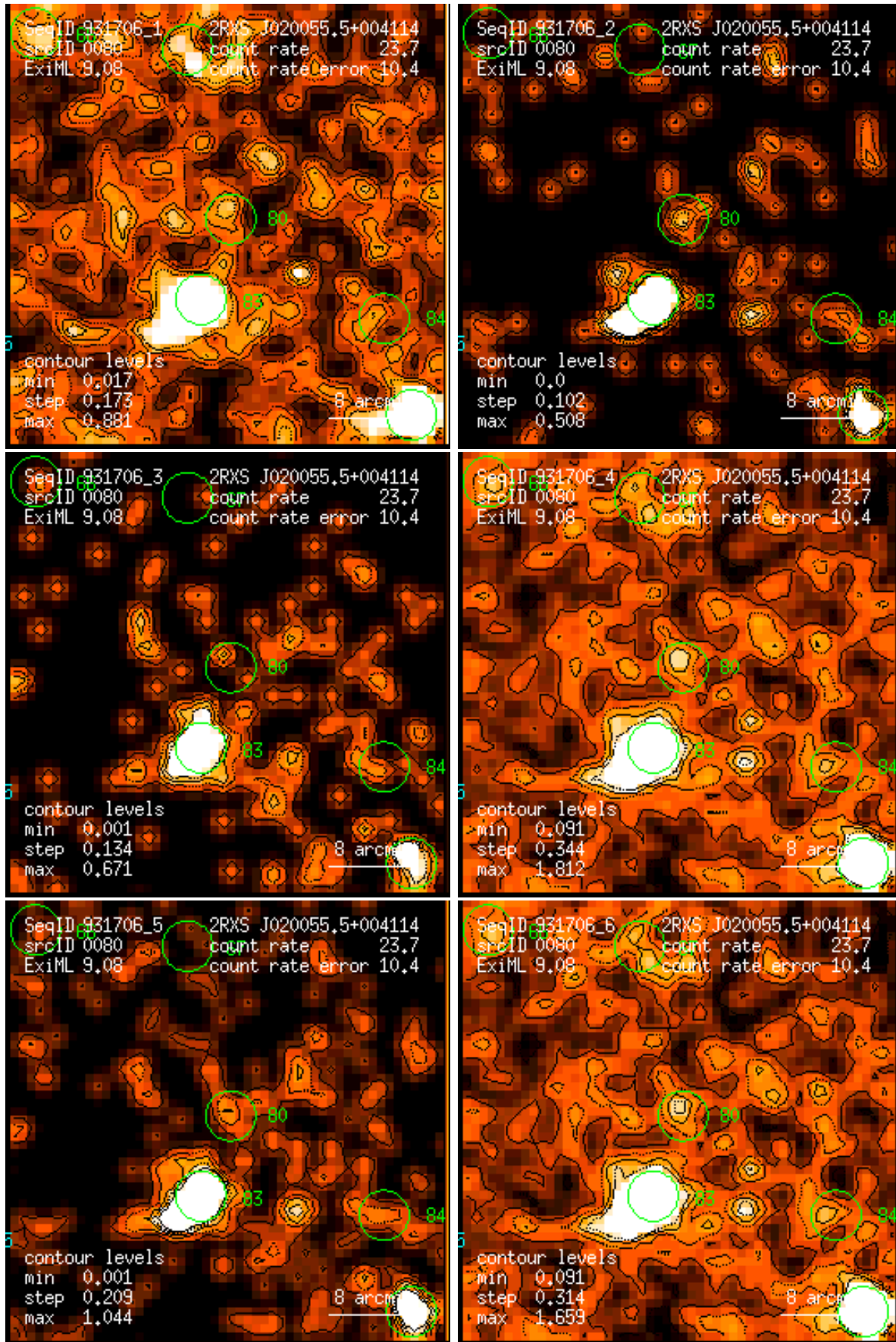
Figure 80: RASS 931706: detection 0080: band rate images, Gaussian filter: (1) PSPC channels 11 – 41, (2) 52 – 90, (3) 91 – 201, (4) 11 – 235, (5) 52 – 201, (6) 11 – 201. Broad band rates in counts/ks. Band rate contour levels in counts/ks/arcmin 2 .
