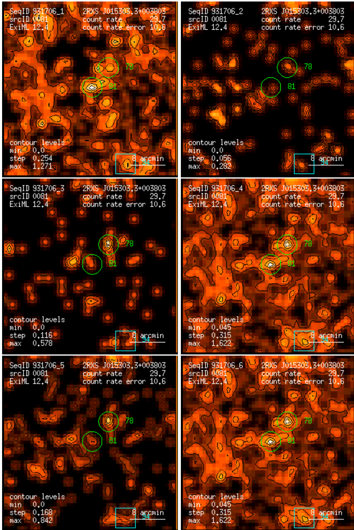
Figure 81: RASS 931706: detection 0081: band rate images, Gaussian filter: (1) PSPC channels 11 – 41, (2) 52 – 90, (3) 91 – 201, (4) 11 – 235, (5) 52 – 201, (6) 11 – 201. Broad band rates in counts/ks. Band rate contour levels in counts/ks/arcmin 2 .
