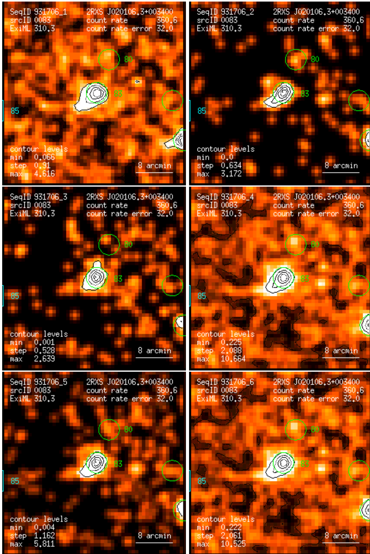
Figure 83: RASS 931706: detection 0083: band rate images, Gaussian filter: (1) PSPC channels 11 – 41, (2) 52 – 90, (3) 91 – 201, (4) 11 – 235, (5) 52 – 201, (6) 11 – 201. Broad band rates in counts/ks. Band rate contour levels in counts/ks/arcmin 2 .
