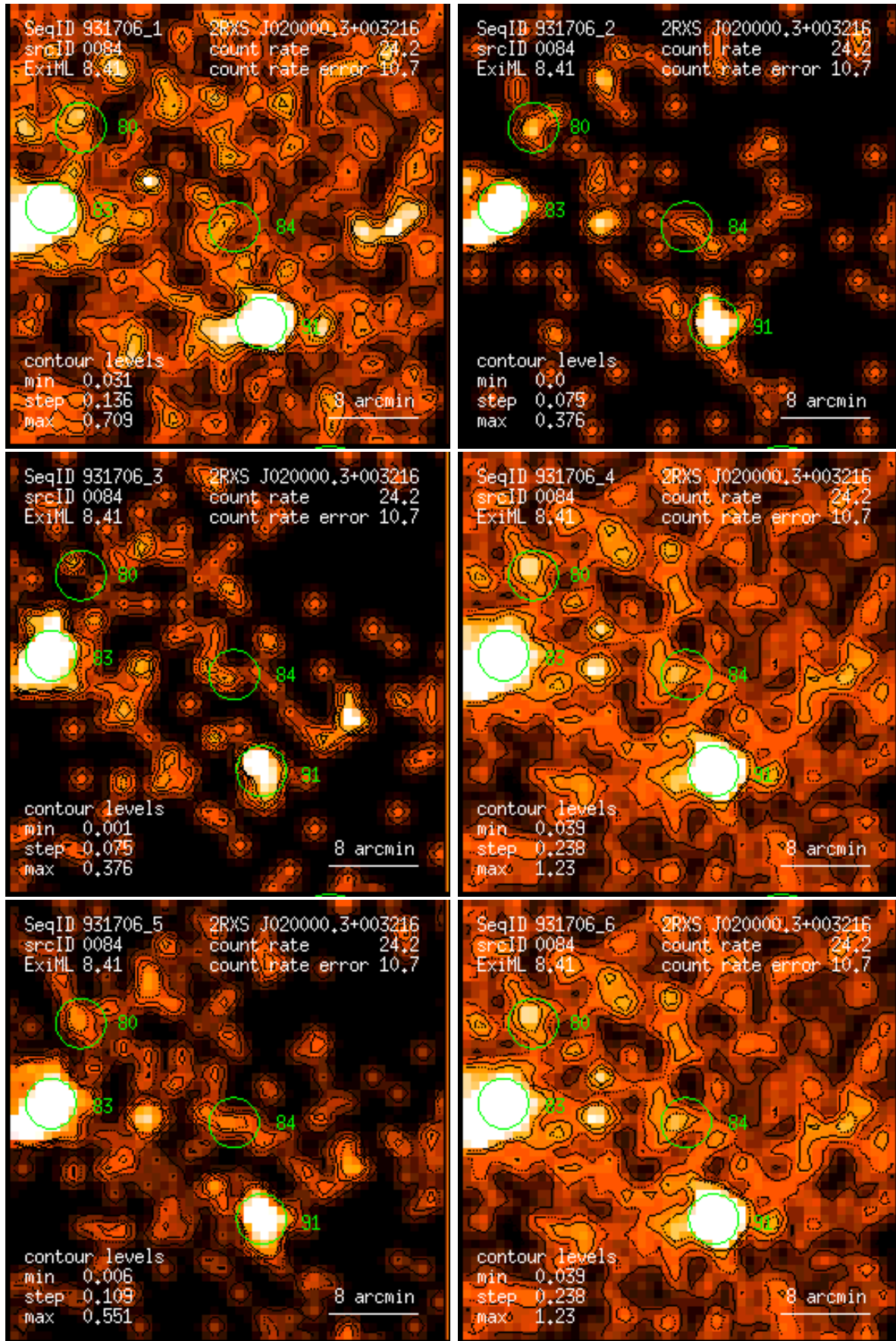
Figure 84: RASS 931706: detection 0084: band rate images, Gaussian filter: (1) PSPC channels 11 – 41, (2) 52 – 90, (3) 91 – 201, (4) 11 – 235, (5) 52 – 201, (6) 11 – 201. Broad band rates in counts/ks. Band rate contour levels in counts/ks/arcmin 2 .
