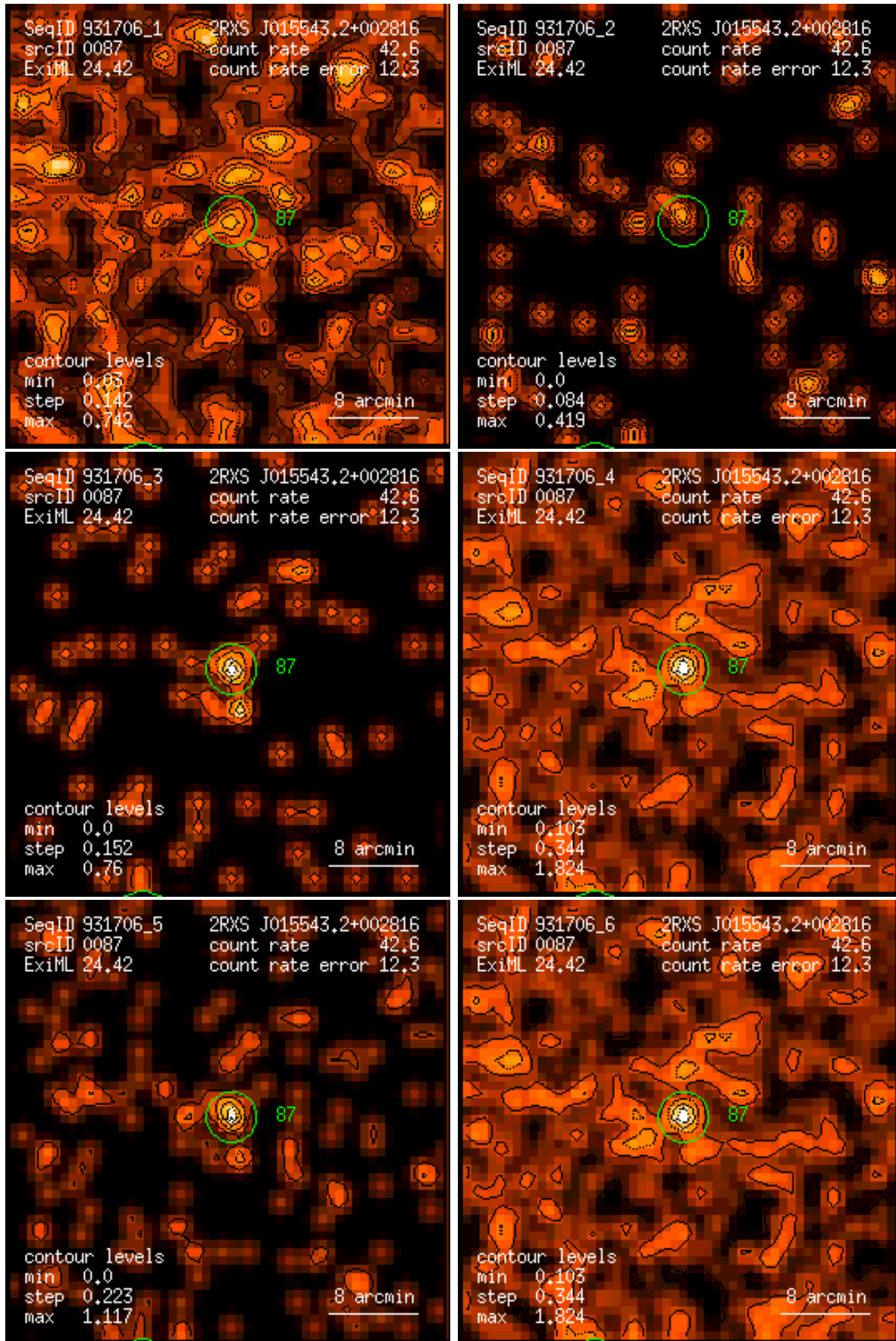
Figure 87: RASS 931706: detection 0087: band rate images, Gaussian filter: (1) PSPC channels 11 – 41, (2) 52 – 90, (3) 91 – 201, (4) 11 – 235, (5) 52 – 201, (6) 11 – 201. Broad band rates in counts/ks. Band rate contour levels in counts/ks/arcmin 2 .
