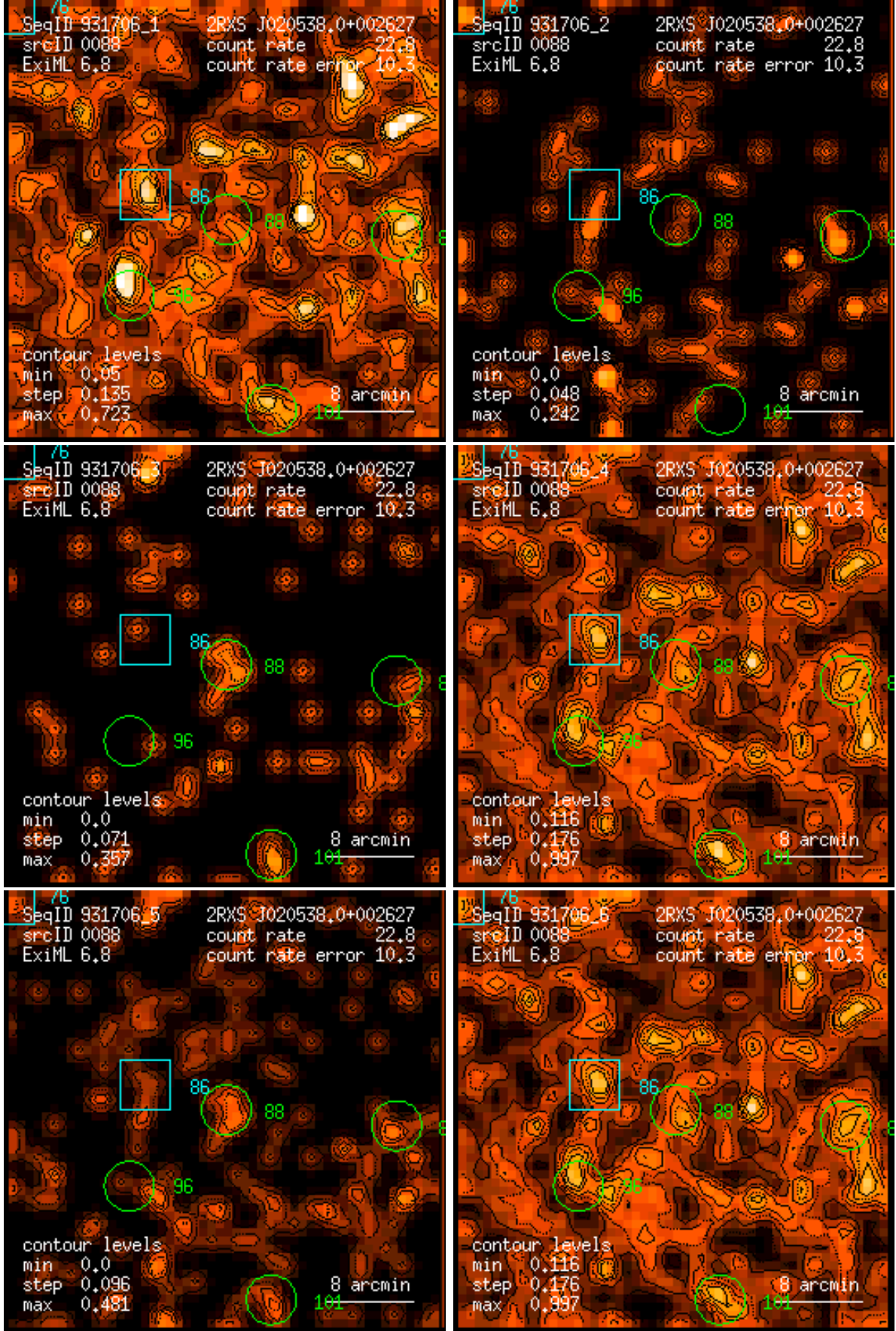
Figure 88: RASS 931706: detection 0088: band rate images, Gaussian filter: (1) PSPC channels 11 – 41, (2) 52 – 90, (3) 91 – 201, (4) 11 – 235, (5) 52 – 201, (6) 11 – 201. Broad band rates in counts/ks. Band rate contour levels in counts/ks/arcmin 2 .
