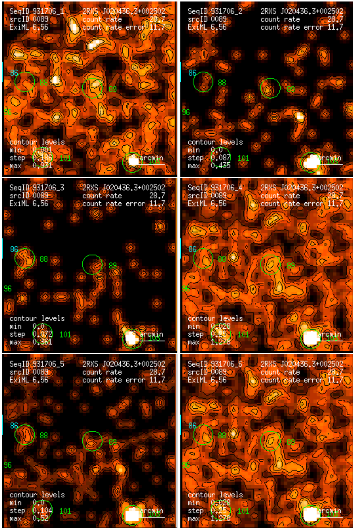
Figure 89: RASS 931706: detection 0089: band rate images, Gaussian filter: (1) PSPC channels 11 – 41, (2) 52 – 90, (3) 91 – 201, (4) 11 – 235, (5) 52 – 201, (6) 11 – 201. Broad band rates in counts/ks. Band rate contour levels in counts/ks/arcmin 2 .
