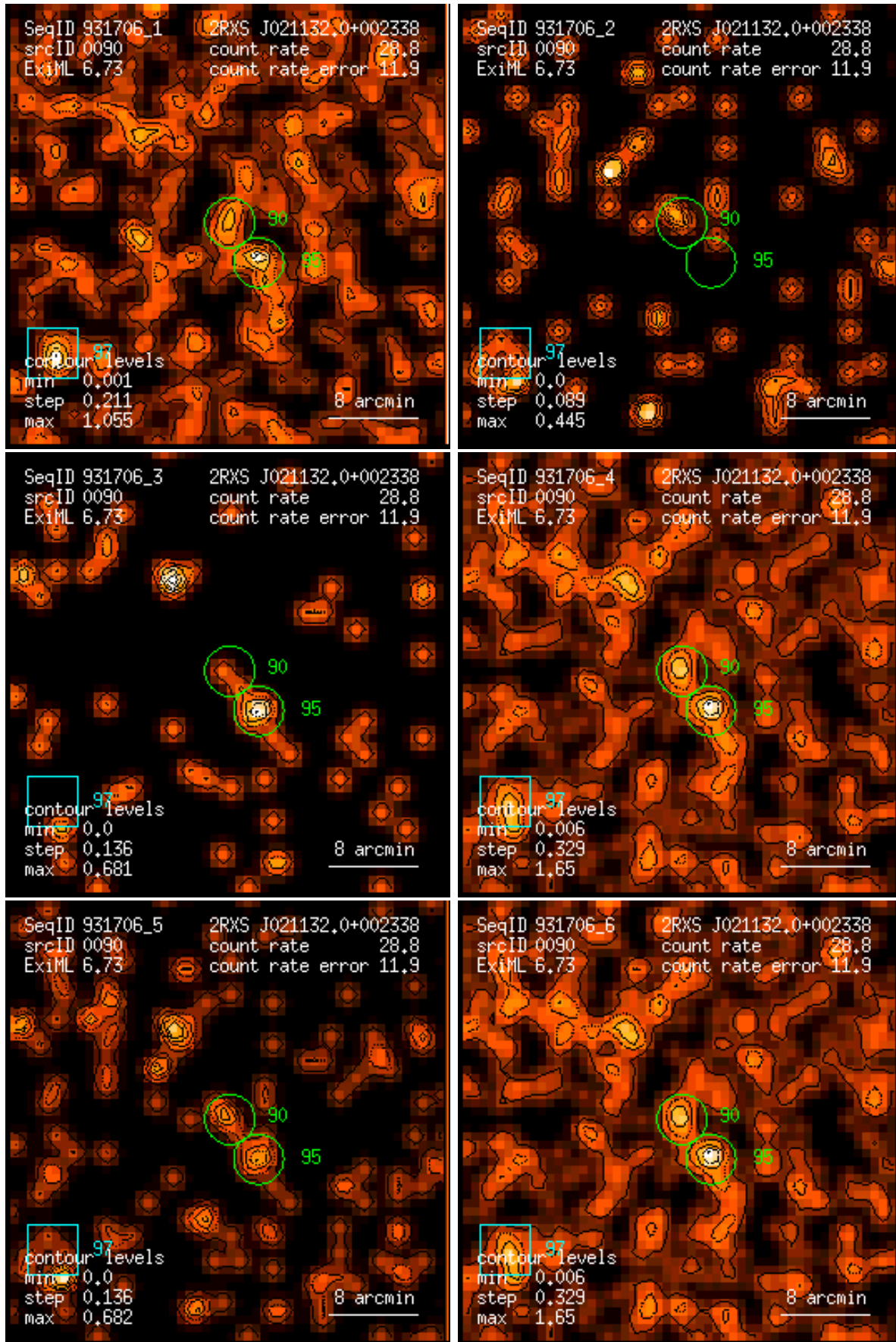
Figure 90: RASS 931706: detection 0090: band rate images, Gaussian filter: (1) PSPC channels 11 – 41, (2) 52 – 90, (3) 91 – 201, (4) 11 – 235, (5) 52 – 201, (6) 11 – 201. Broad band rates in counts/ks. Band rate contour levels in counts/ks/arcmin 2 .
