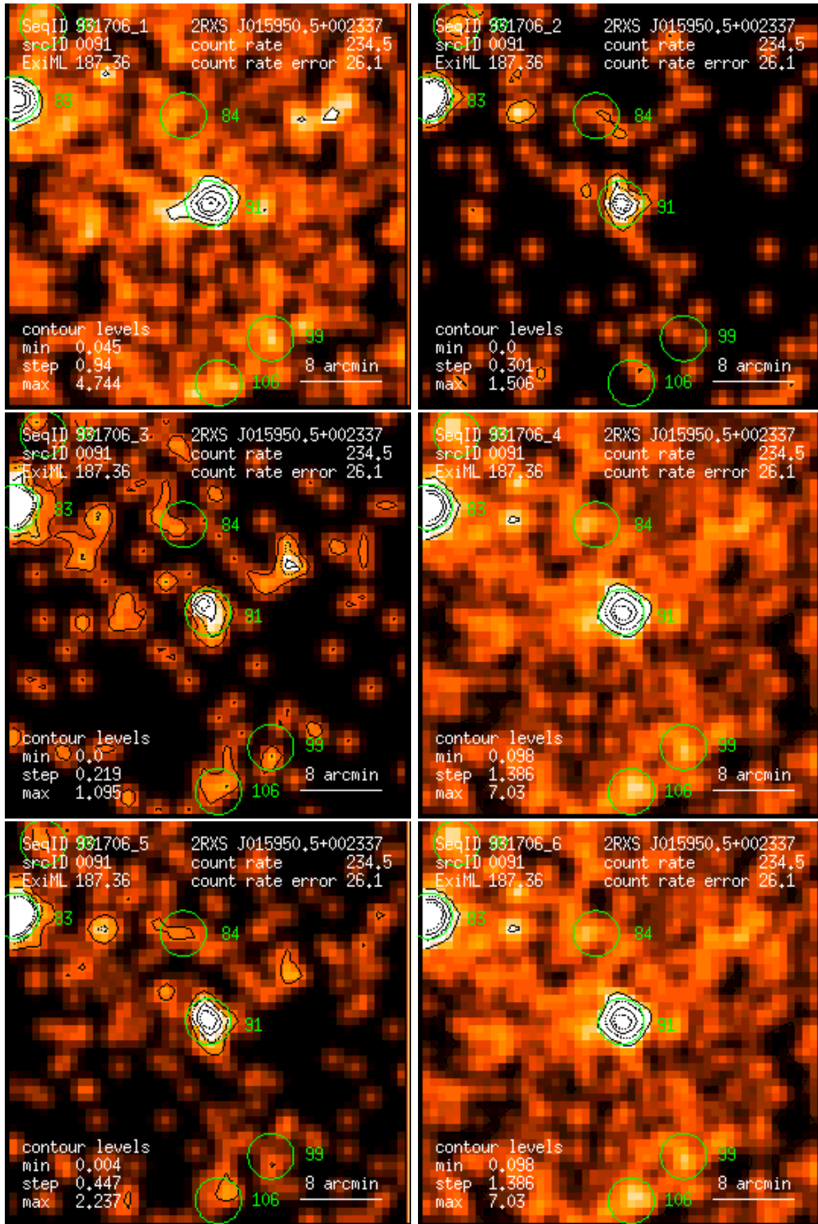
Figure 91: RASS 931706: detection 0091: band rate images, Gaussian filter: (1) PSPC channels 11 – 41, (2) 52 – 90, (3) 91 – 201, (4) 11 – 235, (5) 52 – 201, (6) 11 – 201. Broad band rates in counts/ks. Band rate contour levels in counts/ks/arcmin 2 .
