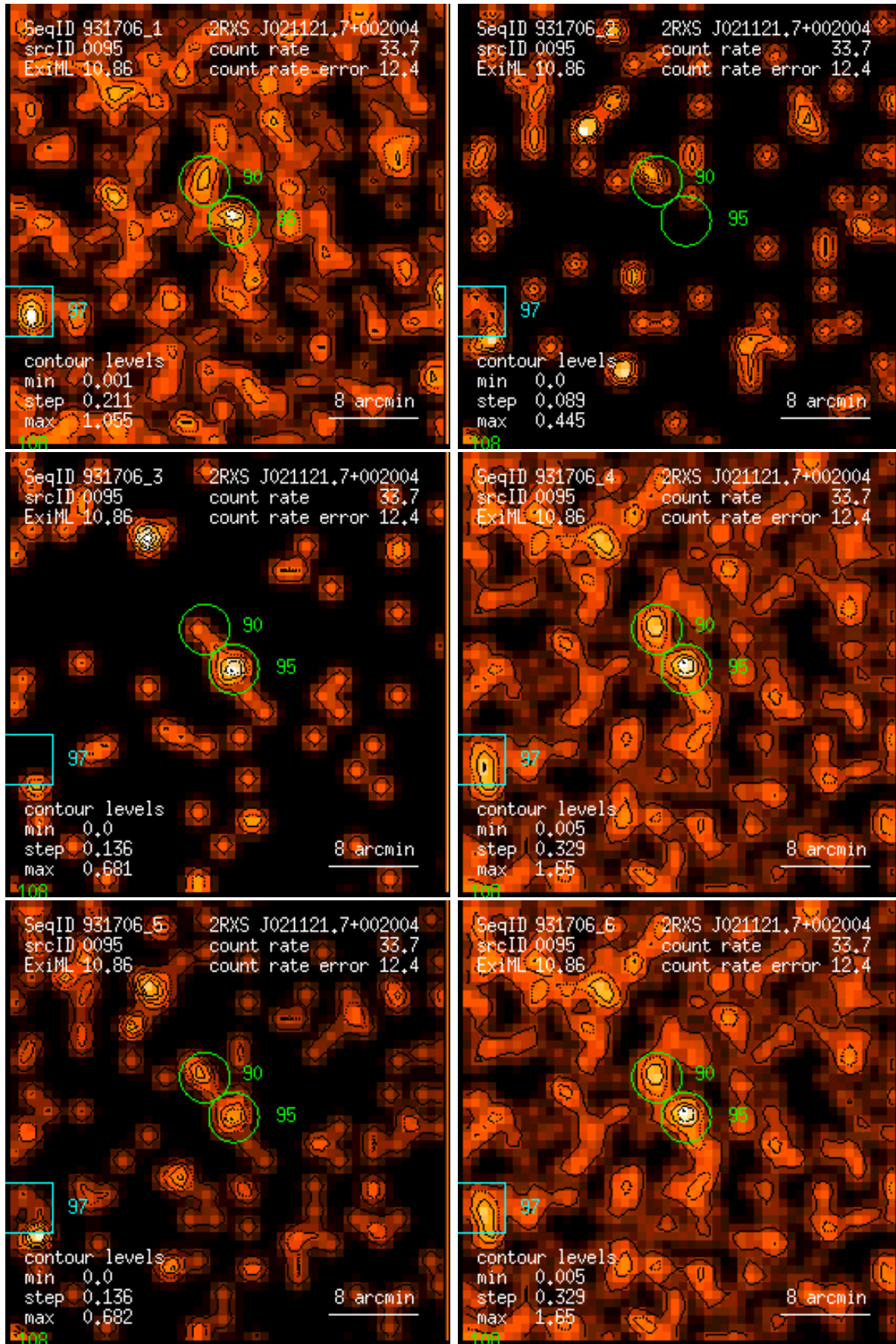
Figure 95: RASS 931706: detection 0095: band rate images, Gaussian filter: (1) PSPC channels 11 – 41, (2) 52 – 90, (3) 91 – 201, (4) 11 – 235, (5) 52 – 201, (6) 11 – 201. Broad band rates in counts/ks. Band rate contour levels in counts/ks/arcmin 2 .
