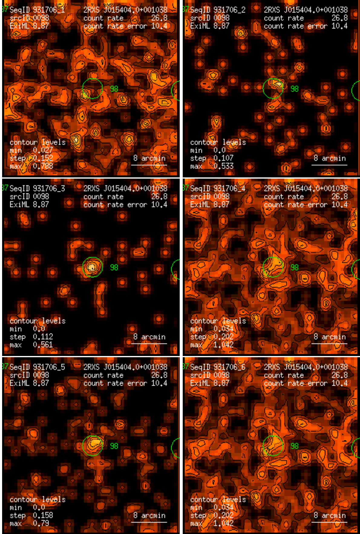
Figure 98: RASS 931706: detection 0098: band rate images, Gaussian filter: (1) PSPC channels 11 – 41, (2) 52 – 90, (3) 91 – 201, (4) 11 – 235, (5) 52 – 201, (6) 11 – 201. Broad band rates in counts/ks. Band rate contour levels in counts/ks/arcmin 2 .
