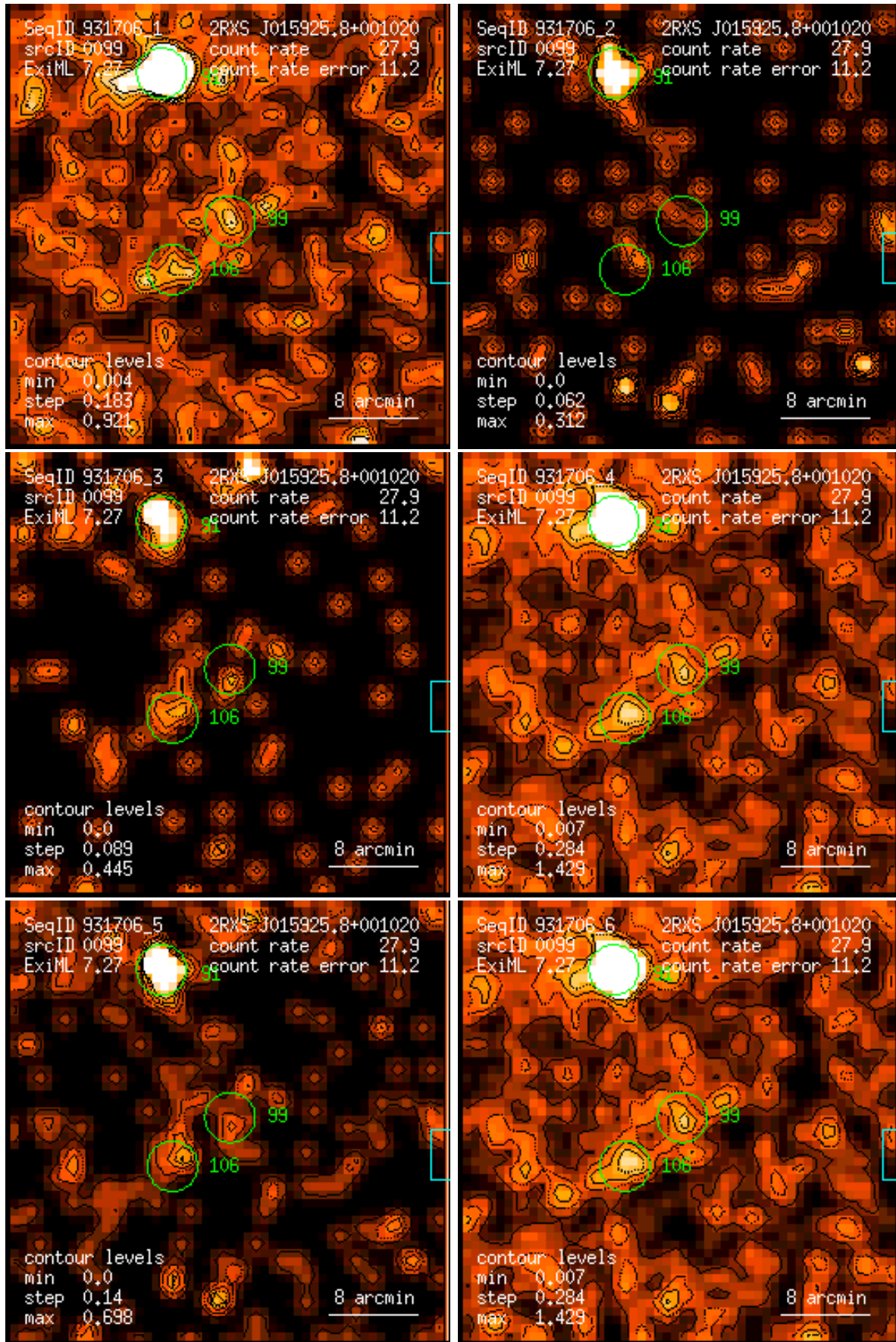
Figure 99: RASS 931706: detection 0099: band rate images, Gaussian filter: (1) PSPC channels 11 – 41, (2) 52 – 90, (3) 91 – 201, (4) 11 – 235, (5) 52 – 201, (6) 11 – 201. Broad band rates in counts/ks. Band rate contour levels in counts/ks/arcmin 2 .
