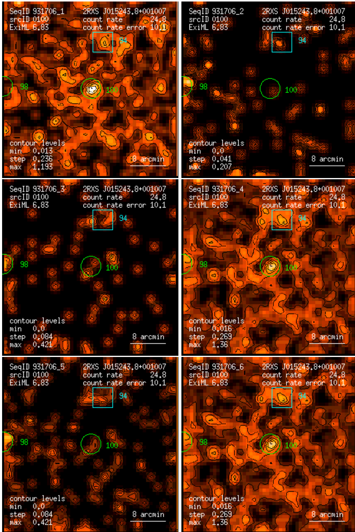
Figure 100: RASS 931706: detection 0100: band rate images, Gaussian filter: (1) PSPC channels 11 – 41, (2) 52 – 90, (3) 91 – 201, (4) 11 – 235, (5) 52 – 201, (6) 11 – 201. Broad band rates in counts/ks. Band rate contour levels in counts/ks/arcmin 2 .
