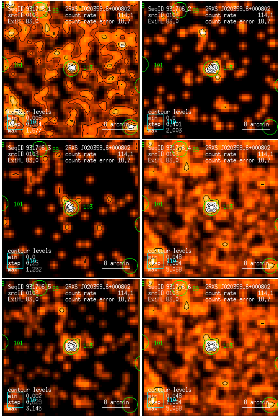
Figure 103: RASS 931706: detection 0103: band rate images, Gaussian filter: (1) PSPC channels 11 – 41, (2) 52 – 90, (3) 91 – 201, (4) 11 – 235, (5) 52 – 201, (6) 11 – 201. Broad band rates in counts/ks. Band rate contour levels in counts/ks/arcmin 2 .
