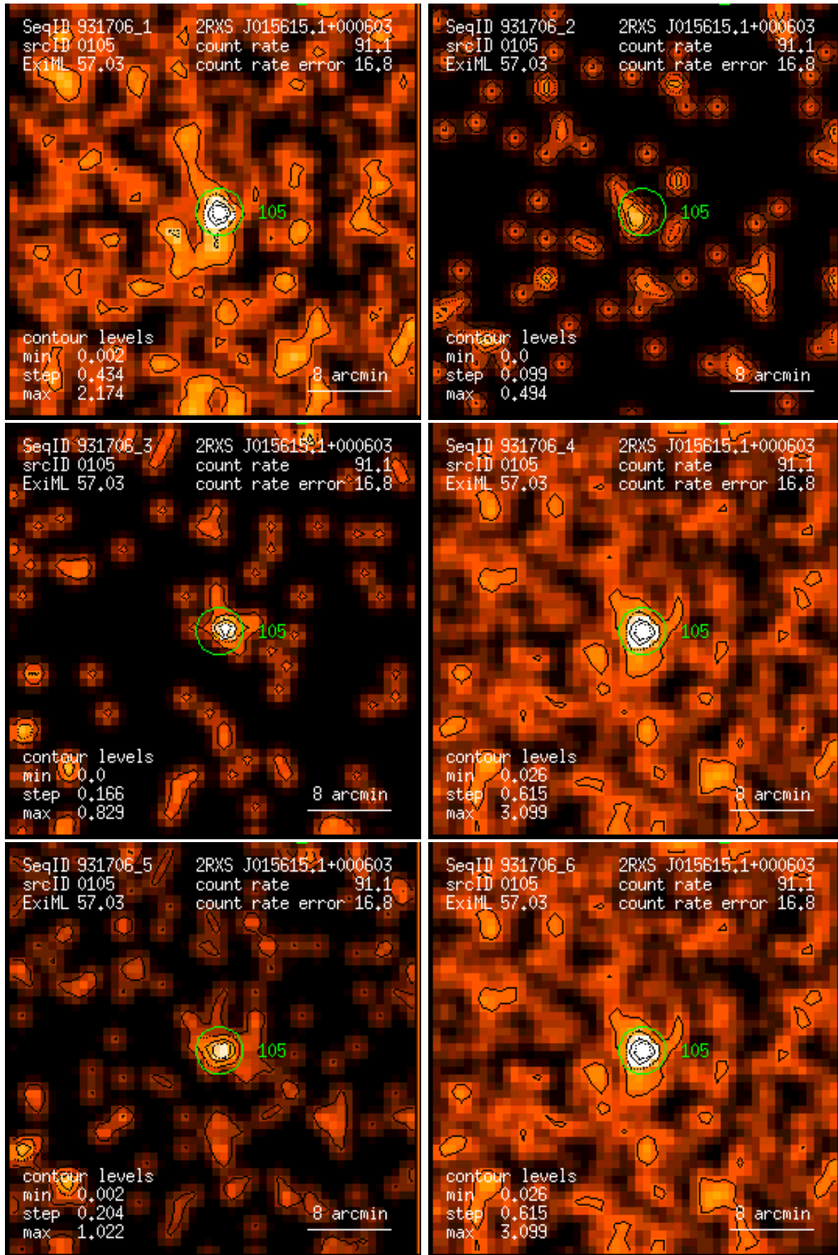
Figure 105: RASS 931706: detection 0105: band rate images, Gaussian filter: (1) PSPC channels 11 – 41, (2) 52 – 90, (3) 91 – 201, (4) 11 – 235, (5) 52 – 201, (6) 11 – 201. Broad band rates in counts/ks. Band rate contour levels in counts/ks/arcmin 2 .
