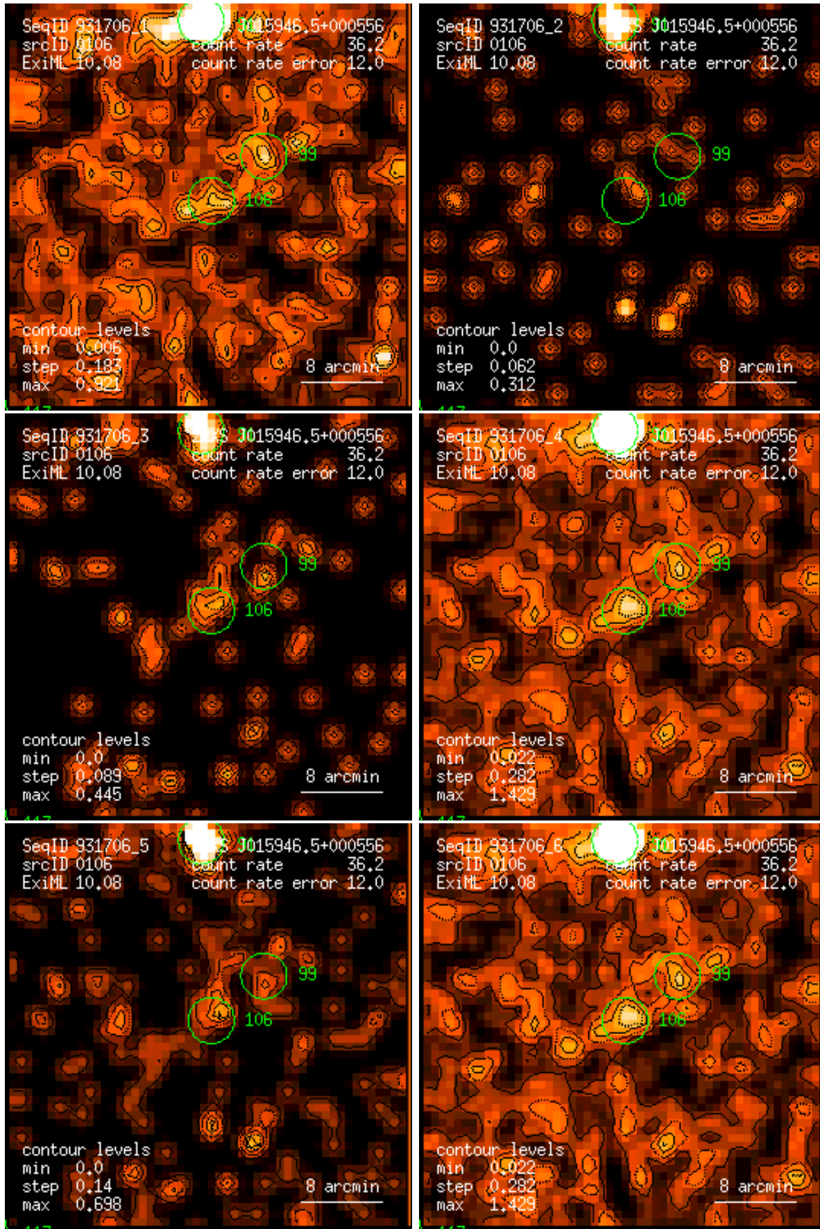
Figure 106: RASS 931706: detection 0106: band rate images, Gaussian filter: (1) PSPC channels 11 – 41, (2) 52 – 90, (3) 91 – 201, (4) 11 – 235, (5) 52 – 201, (6) 11 – 201. Broad band rates in counts/ks. Band rate contour levels in counts/ks/arcmin 2 .
