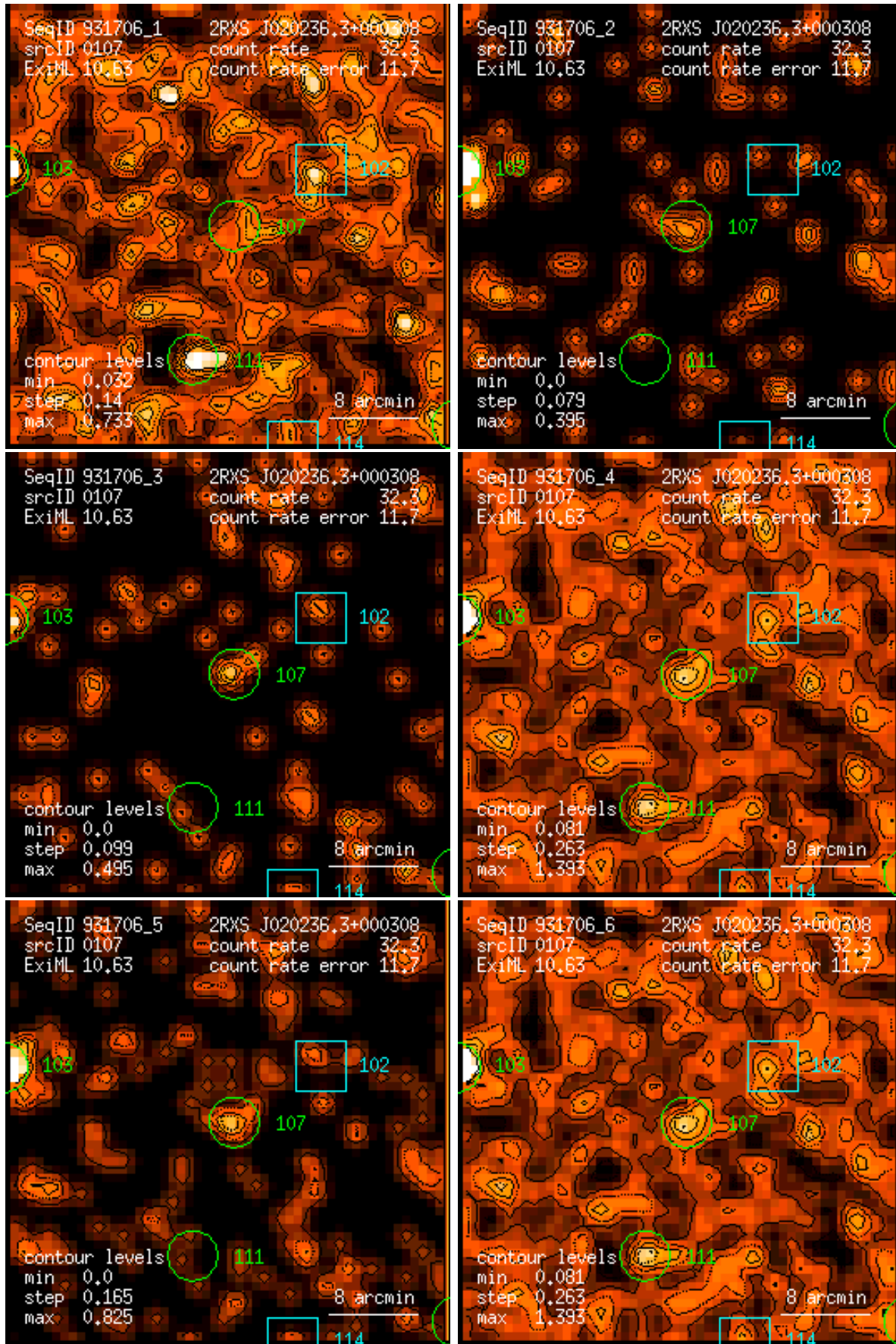
Figure 107: RASS 931706: detection 0107: band rate images, Gaussian filter: (1) PSPC channels 11 – 41, (2) 52 – 90, (3) 91 – 201, (4) 11 – 235, (5) 52 – 201, (6) 11 – 201. Broad band rates in counts/ks. Band rate contour levels in counts/ks/arcmin 2 .
