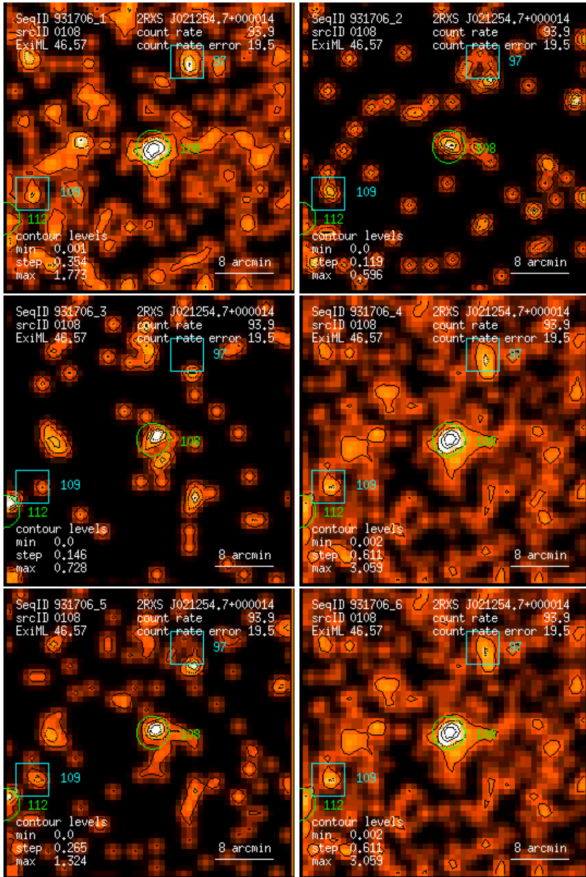
Figure 108: RASS 931706: detection 0108: band rate images, Gaussian filter: (1) PSPC channels 11 – 41, (2) 52 – 90, (3) 91 – 201, (4) 11 – 235, (5) 52 – 201, (6) 11 – 201. Broad band rates in counts/ks. Band rate contour levels in counts/ks/arcmin 2 .
