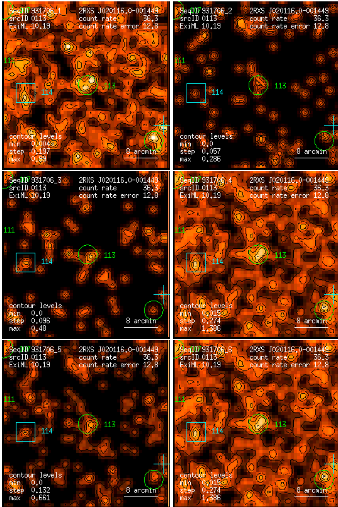
Figure 113: RASS 931706: detection 0113: band rate images, Gaussian filter: (1) PSPC channels 11 – 41, (2) 52 – 90, (3) 91 – 201, (4) 11 – 235, (5) 52 – 201, (6) 11 – 201. Broad band rates in counts/ks. Band rate contour levels in counts/ks/arcmin 2 .
